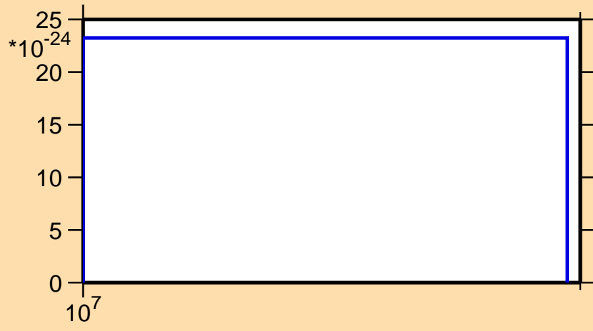
\sigma vs. E for ^{146}\text{Ba} (mt 11)
