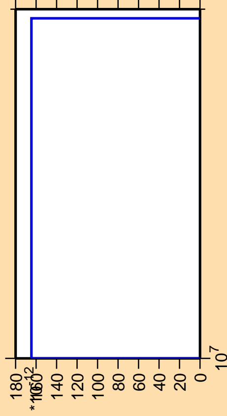
\Delta\sigma/\sigma vs. E for ^{146}\text{Ba} (mt 11)
