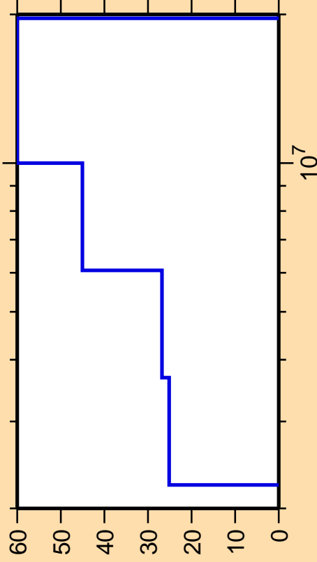
\Delta\sigma/\sigma vs. E for ^{146}\text{Ba}(n,n\text{cont.})
