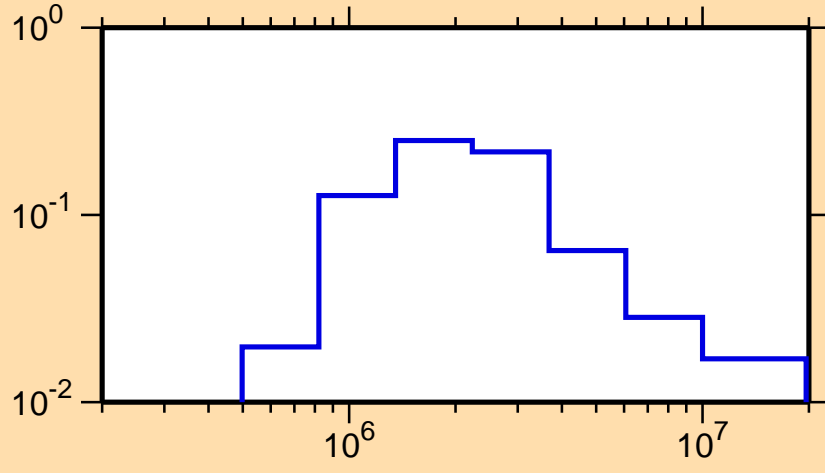
\sigma vs. E for ^{146}\text{Ba}(n,n_2)
