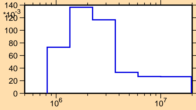
\sigma vs. E for ^{146}\text{Ba}(n,n_4)
