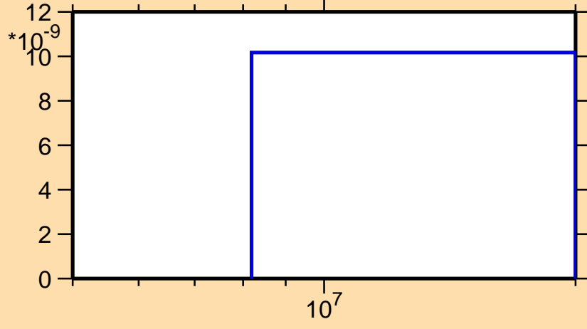
\sigma vs. E for {}^7\text{Be}(n,2np)
