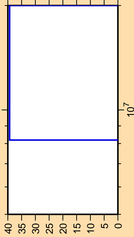
\Delta\sigma/\sigma vs. E for {}^7\text{Be}(n,pd)
