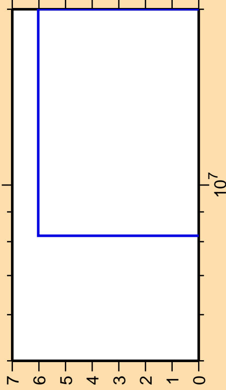
\Delta\sigma/\sigma vs. E for {}^7\text{Be}(n,\alpha)
