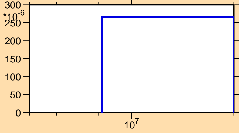
\sigma vs. E for {}^7\text{Be}(n,pd)
