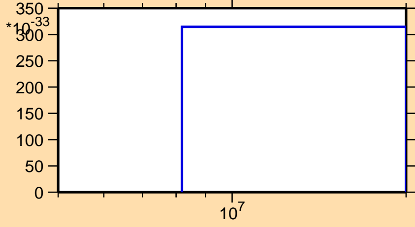
\sigma vs. E for ^{11}\text{Be}(n,2n\alpha)
