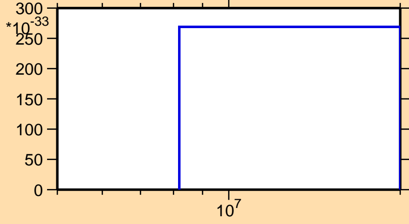
\sigma vs. E for ^{11}\text{Be}(n,n\alpha)
