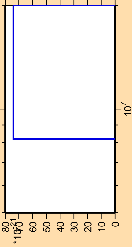
\Delta\sigma/\sigma vs. E for ^{11}\text{Be}(n,2n\alpha)
