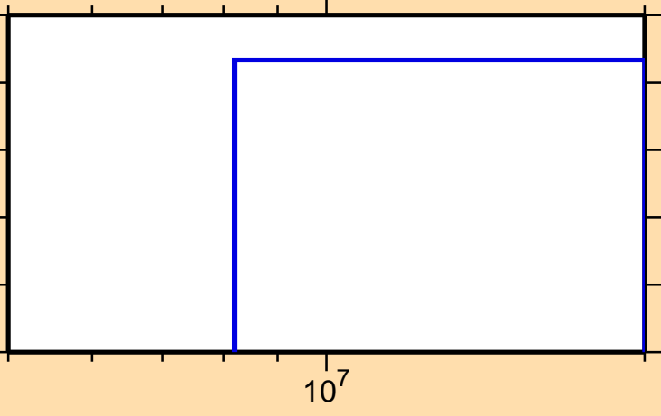
\sigma vs. E for ^{11}\text{Be}(n,nt)
