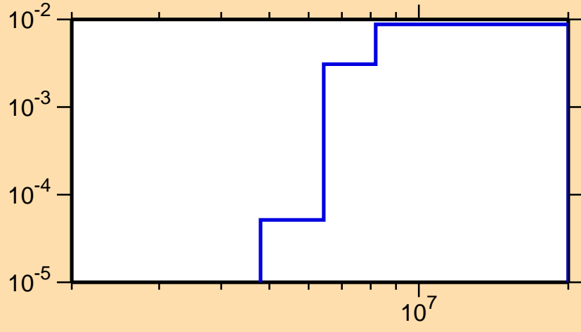
\sigma vs. E for ^{11}\text{Be}(n,\alpha)
