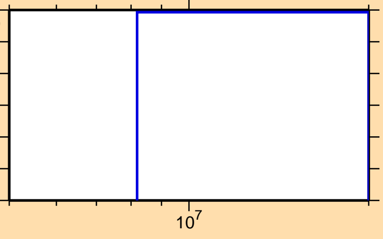
\sigma vs. E for ^{11}\text{Be}(n,nd)
