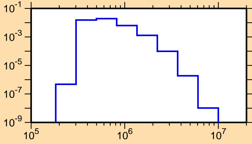
\sigma vs. E for ^{264}_{1}
