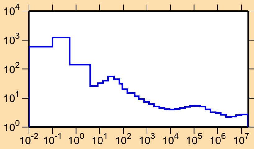
\sigma vs. E for ^{266}
