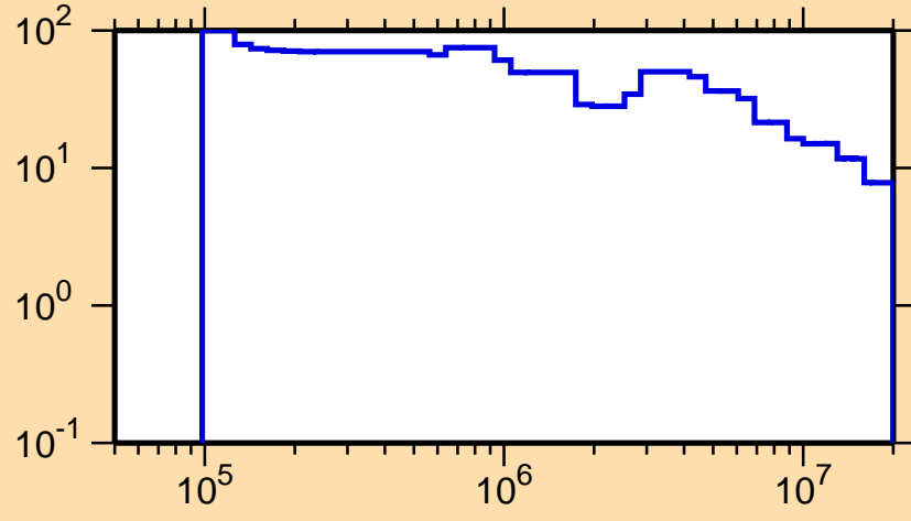
\Delta\sigma/\sigma vs. E for ^{270}_{1}\text{Pb}
