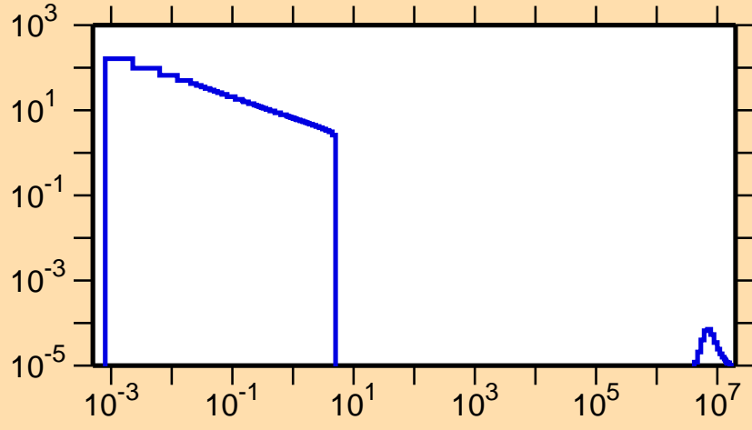
\sigma vs. E for ^{274}\gamma
