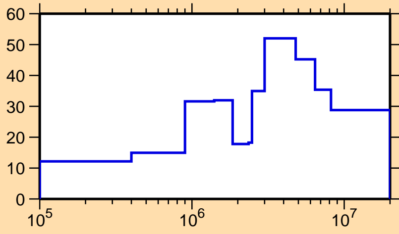
\Delta\sigma/\sigma vs. E for ^{274}_1
