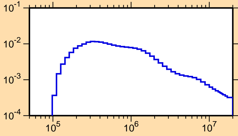
\sigma vs. E for ^{275}_{1}
