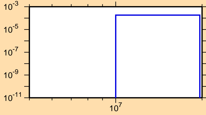
\sigma vs. E for ^{190}\text{Bi}(n,2n\alpha)
