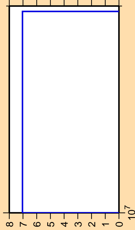
\Delta\sigma/\sigma vs. E for ^{190}\text{Bi}(n,3n\alpha)
