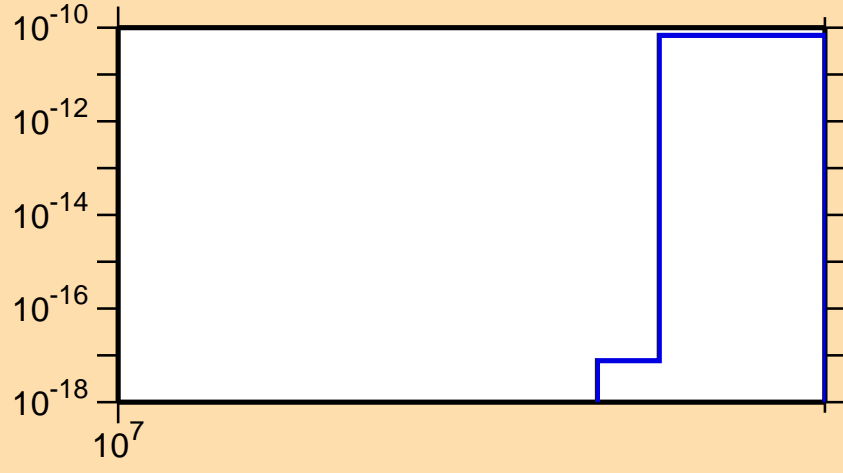
\sigma vs. E for ^{192}\text{Bi}(n,3n\alpha)
