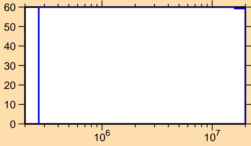
\Delta\sigma/\sigma vs. E for ^{192}\text{Bi}(n,ncont.)
