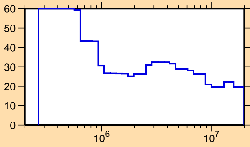
\Delta\sigma/\sigma vs. E for ^{192}\text{Bi}(n,n\text{onel.})
