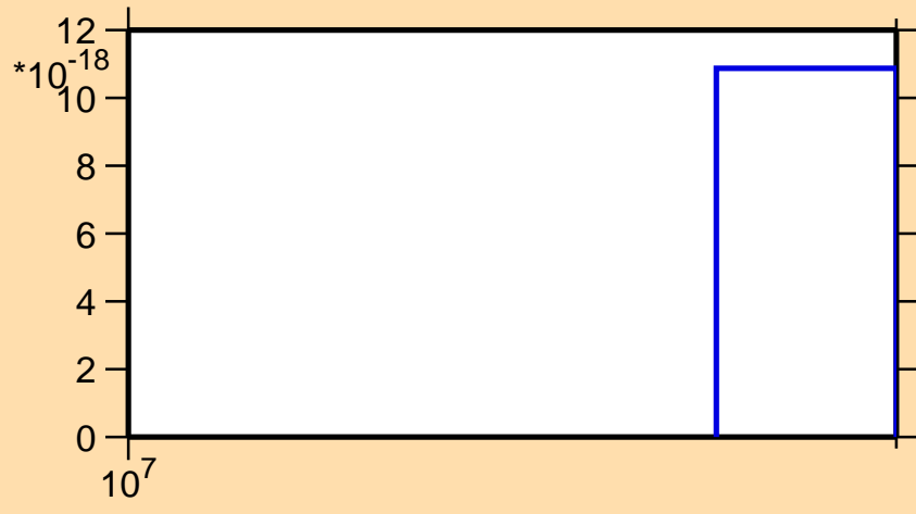
\sigma vs. E for ^{192}\text{Bi} (mt 42)
