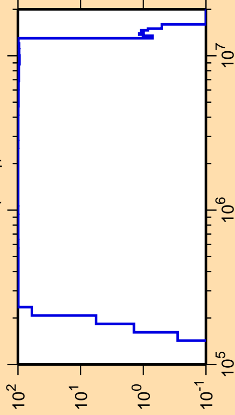
\Delta\sigma/\sigma vs. E for ^{192}\text{Bi}(n,n_1)
