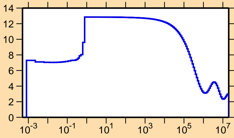
\sigma vs. E for ^{192}\text{Bi}(n,\text{el.})
