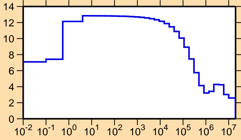
\sigma vs. E for ^{192}\text{Bi}(n,\text{el.})
