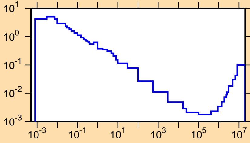
\sigma vs. E for ^{192}\text{Bi}(n,\alpha)
