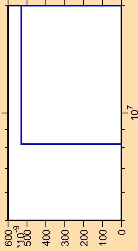
\Delta\sigma/\sigma vs. E for ^{192}\text{Bi}(\text{mt } 42)
