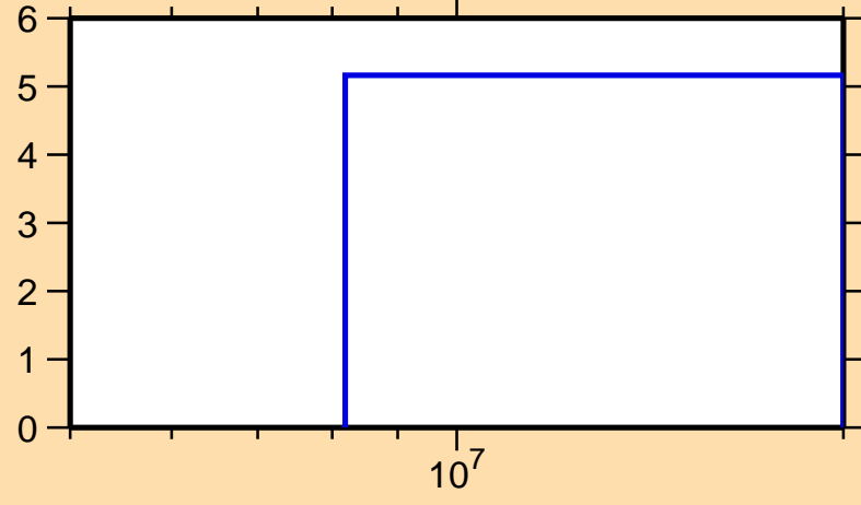
\Delta\sigma/\sigma vs. E for ^{192}\text{Bi}(n,\text{tot.})
