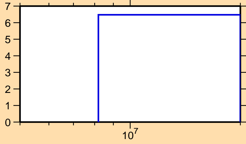
\Delta\sigma/\sigma vs. E for ^{192}\text{Bi}(n,\text{nonel.})
