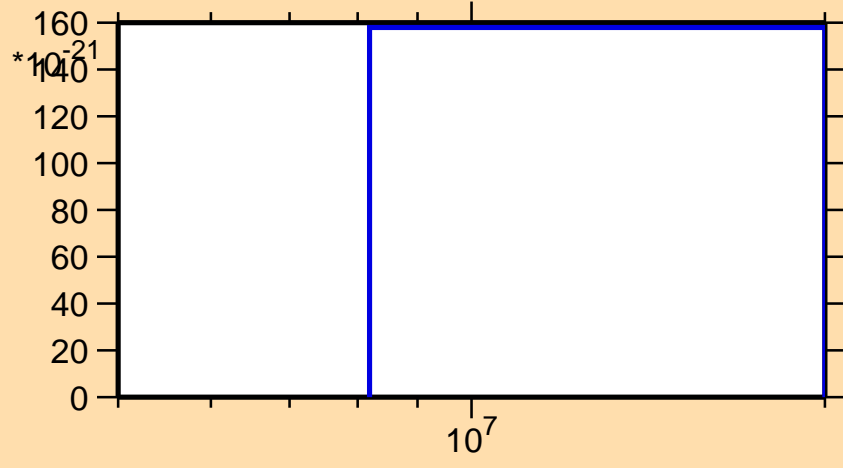
\sigma vs. E for ^{192}\text{Bi}(\text{mt } 42)
