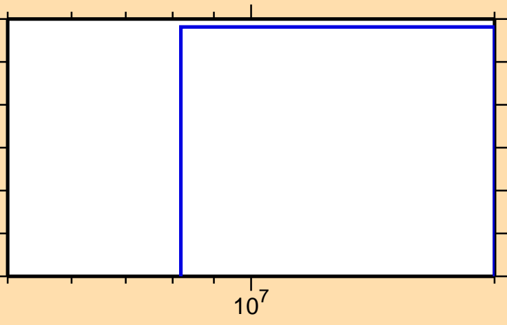
\sigma vs. E for ^{192}\text{Bi}(\text{mt117})
