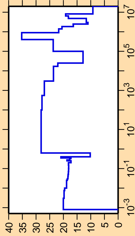
\Delta\sigma/\sigma vs. E for ^{192}\text{Bi}(n,\text{el.})
