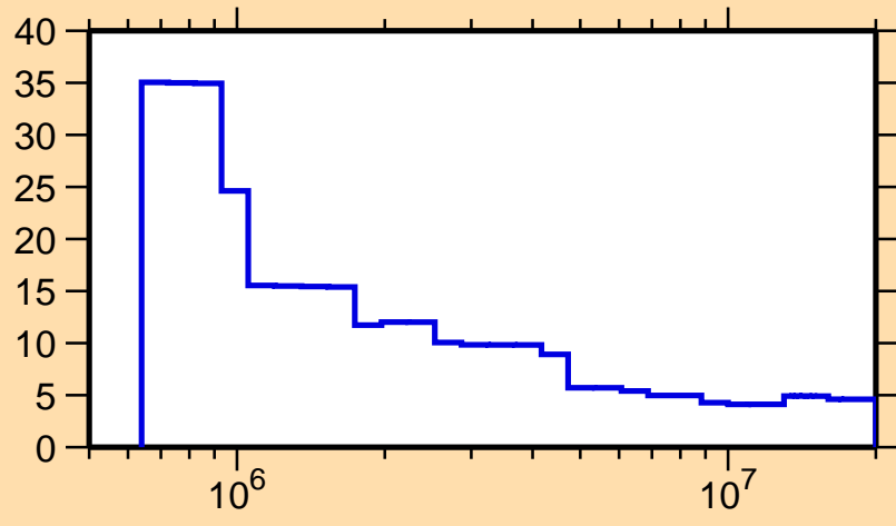
\Delta\sigma/\sigma vs. E for ^{193}\text{Bi}(n,n\text{nonel.})
