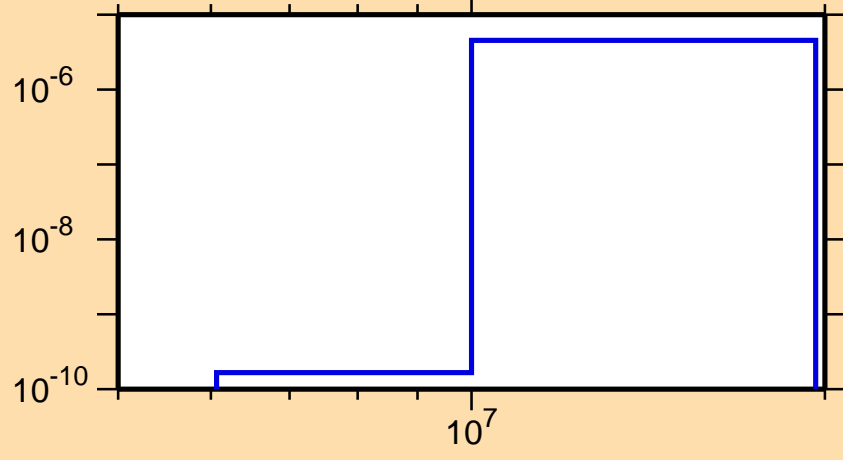
\sigma vs. E for ^{193}\text{Bi} (mt 45)
