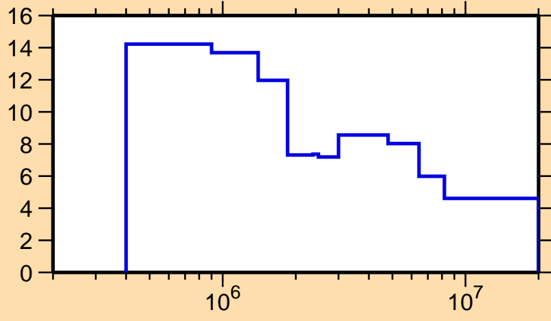
\Delta\sigma/\sigma vs. E for ^{193}\text{Bi}(n,\text{tot.})
