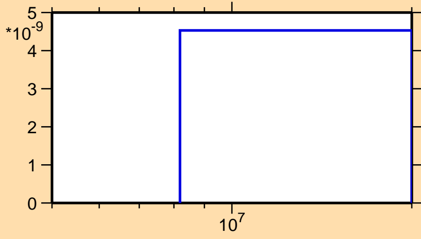
\sigma vs. E for ^{193}\text{Bi}(\text{mt117})
