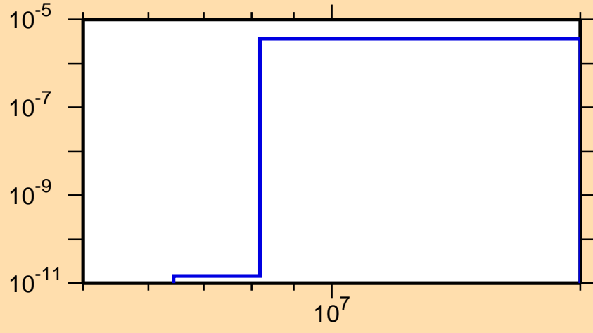
\sigma vs. E for ^{193}\text{Bi} (mt 45)
