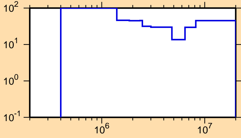
\Delta\sigma/\sigma vs. E for ^{193}\text{Bi}(n,n\text{cont.})
