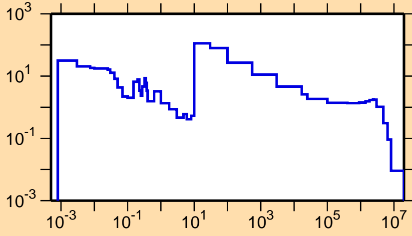
\sigma vs. E for ^{193}\text{Bi}(n,\gamma)
