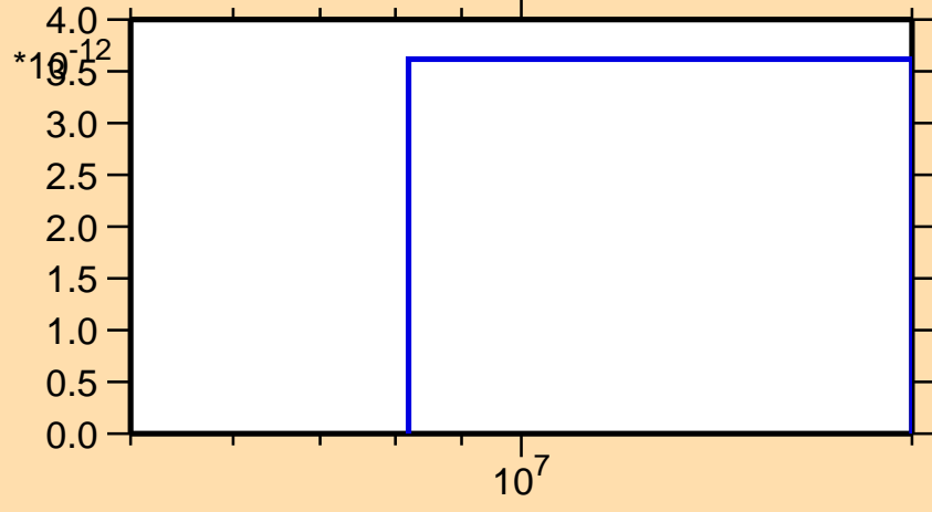
\sigma vs. E for ^{193}\text{Bi} (mt 34)
