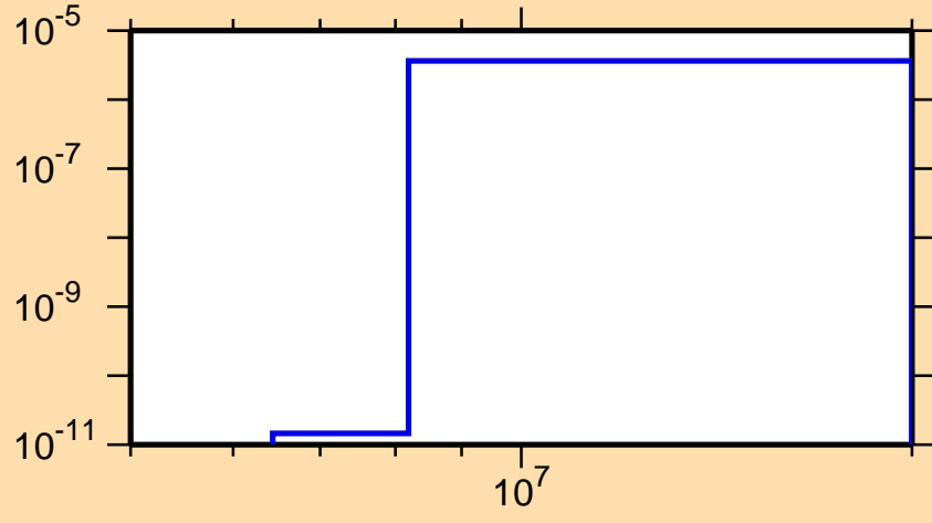
\sigma vs. E for ^{193}\text{Bi}(n,\text{He}3)
