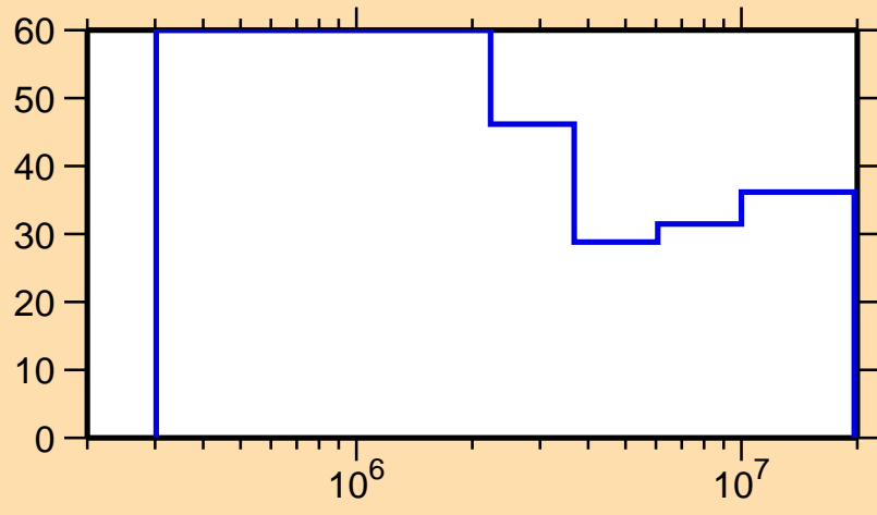
\Delta\sigma/\sigma vs. E for ^{195}\text{Bi}(n,n_1)
