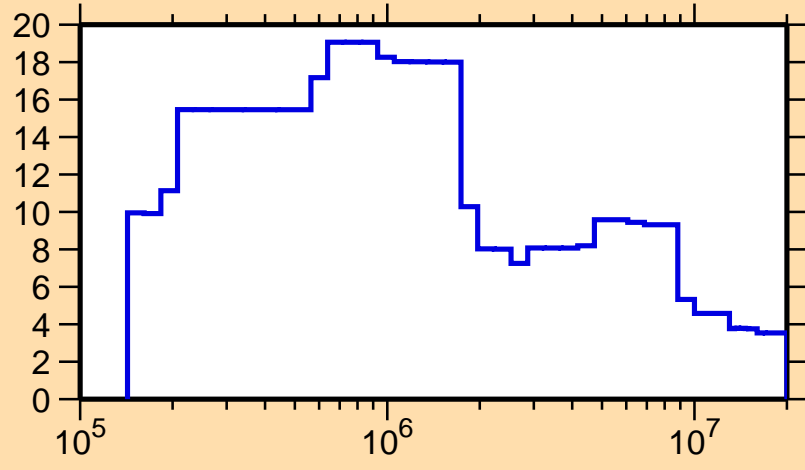
\Delta\sigma/\sigma vs. E for ^{196}\text{Bi}(n,\text{tot.})
