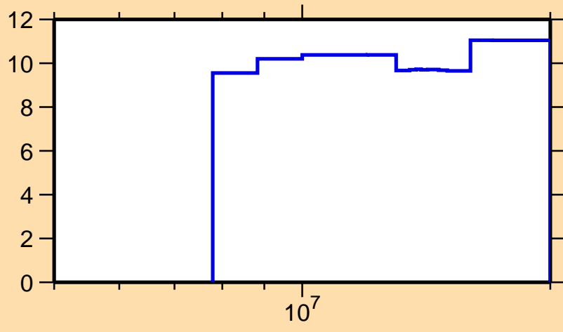
\Delta\sigma/\sigma vs. E for ^{196}\text{Bi}(n,\text{nonel.})
