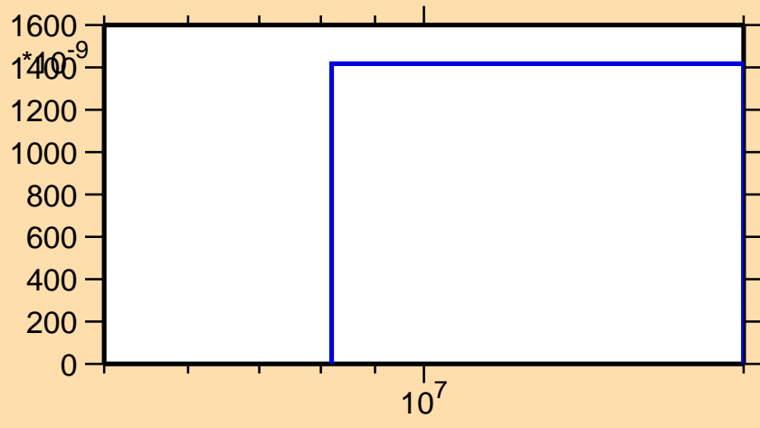
\sigma vs. E for ^{196}\text{Bi}(n,2n\alpha)
