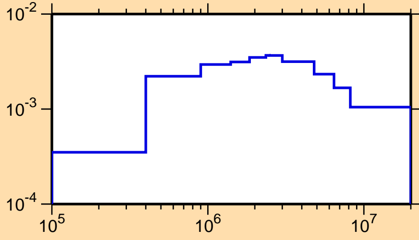
\sigma vs. E for ^{196}\text{Bi}(n,n_1)
