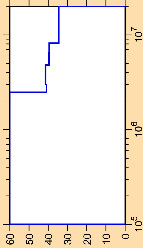
\Delta\sigma/\sigma vs. E for ^{196}\text{Bi}(n,n_1)
