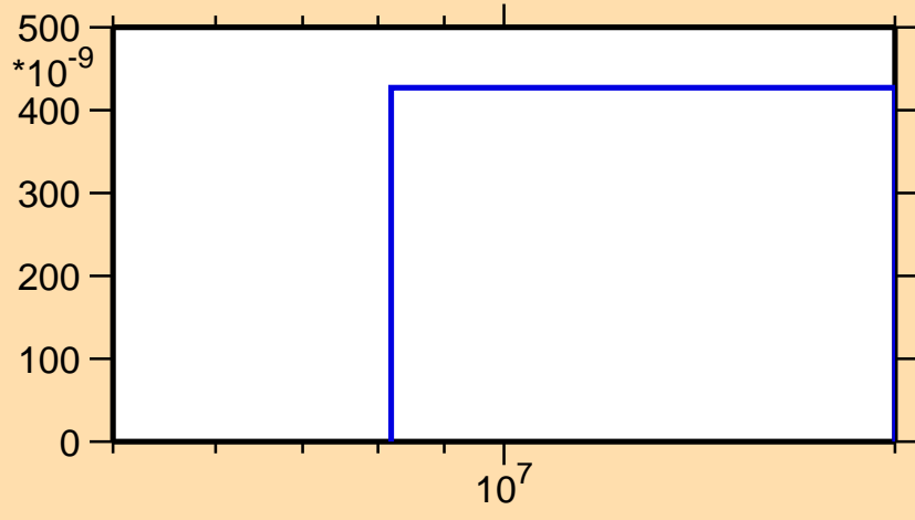
\sigma vs. E for ^{196}\text{Bi}(n,\text{nd})
