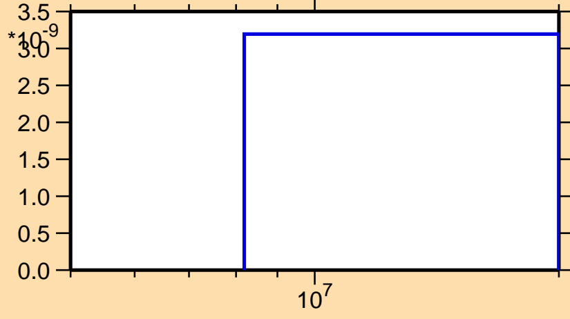
\sigma vs. E for ^{196}\text{Bi} (mt 45)
