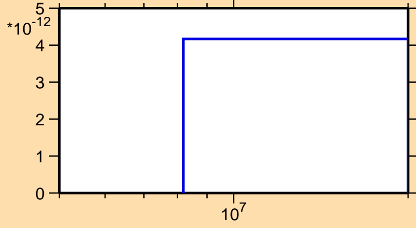
\sigma vs. E for ^{196}\text{Bi} (mt 34)
