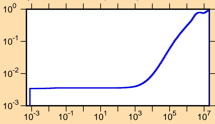
\mu vs. E for ^{197}\text{Bi}(\text{mt251})
