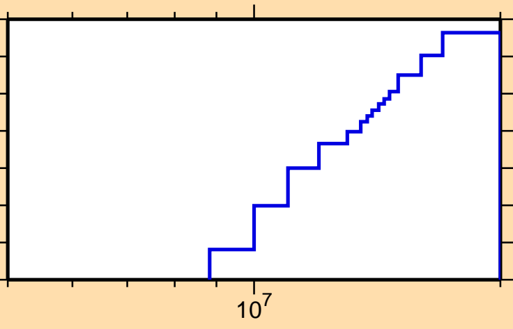
\sigma vs. E for ^{197}\text{Bi}(n,\text{He3})
