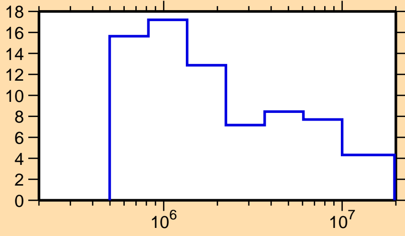
\Delta\sigma/\sigma vs. E for ^{197}\text{Bi}(n,\text{tot.})
