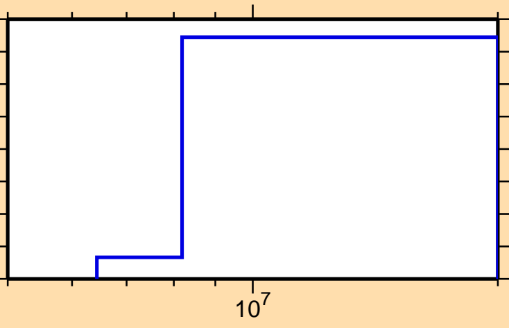
\sigma vs. E for ^{197}\text{Bi}(n,\text{He3})
