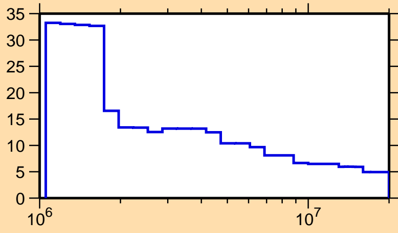
\Delta\sigma/\sigma vs. E for ^{199}\text{Bi}(n,n\text{onel.})
