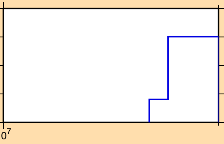
\sigma vs. E for ^{199}\text{Bi}(n,\text{pt})
