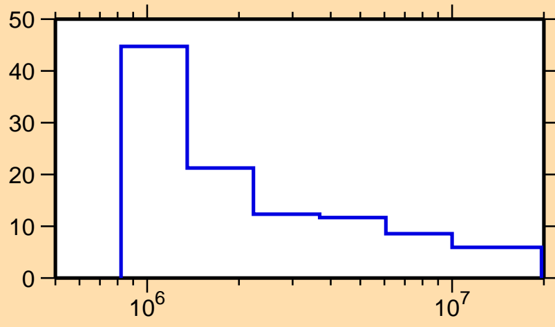
\Delta\sigma/\sigma vs. E for ^{199}\text{Bi}(n,n\text{nonel.})
