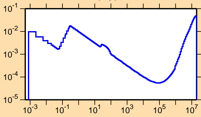
\sigma vs. E for ^{200}\text{Bi}(n,p)
