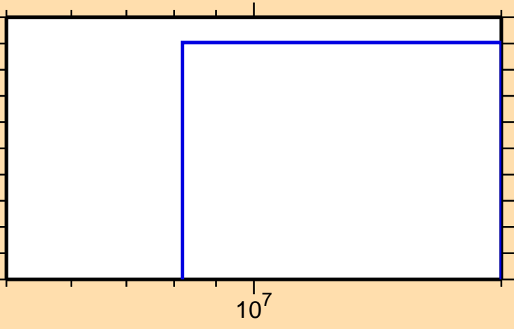
\sigma vs. E for ^{200}\text{Bi}(n,2n\alpha)
