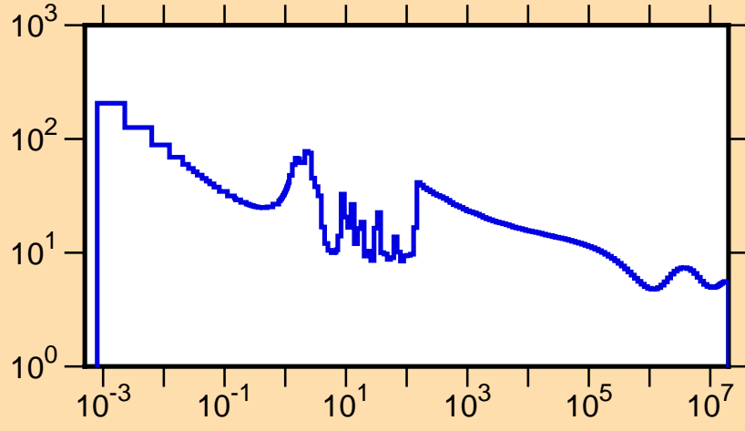
\sigma vs. E for ^{201}\text{Bi}(n,\text{tot.})
