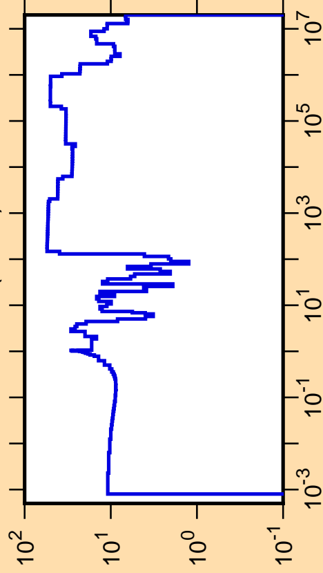
\Delta\sigma/\sigma vs. E for ^{201}\text{Bi}(n,\text{tot.})
