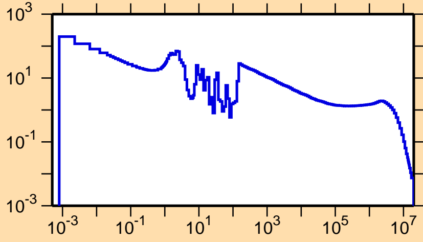
\sigma vs. E for ^{201}\text{Bi}(n,\gamma)
