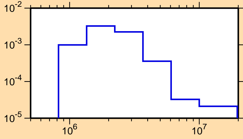
\sigma vs. E for ^{201}\text{Bi}(n,n_1)
