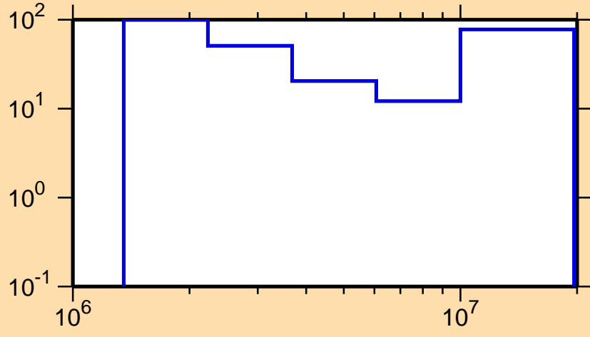
\Delta\sigma/\sigma vs. E for ^{201}\text{Bi}(n,n\text{cont.})
