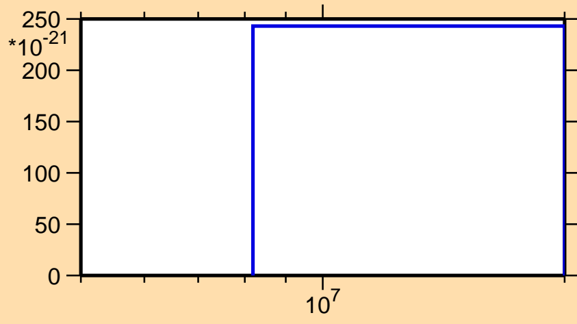
\sigma vs. E for ^{201}\text{Bi} (mt 42)
