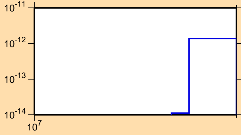
\sigma vs. E for ^{202}\text{Bi} (mt 34)
