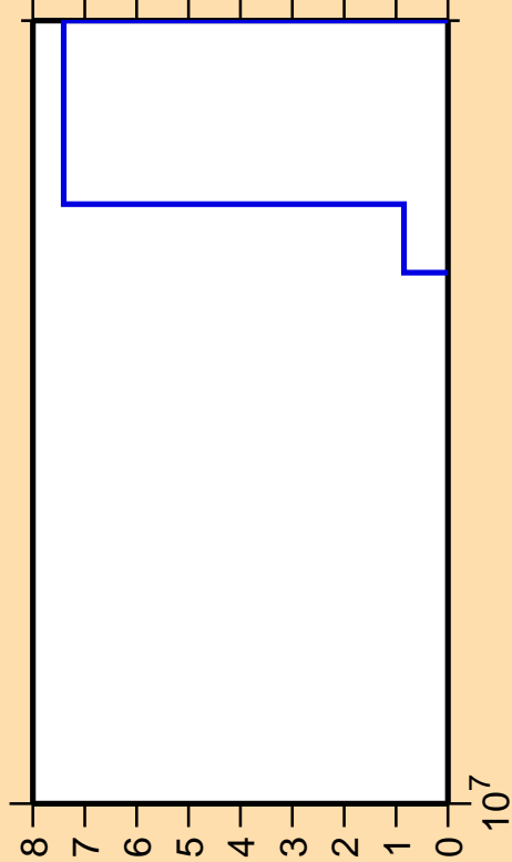
\Delta\sigma/\sigma vs. E for ^{202}\text{Bi}(\text{mt117})
