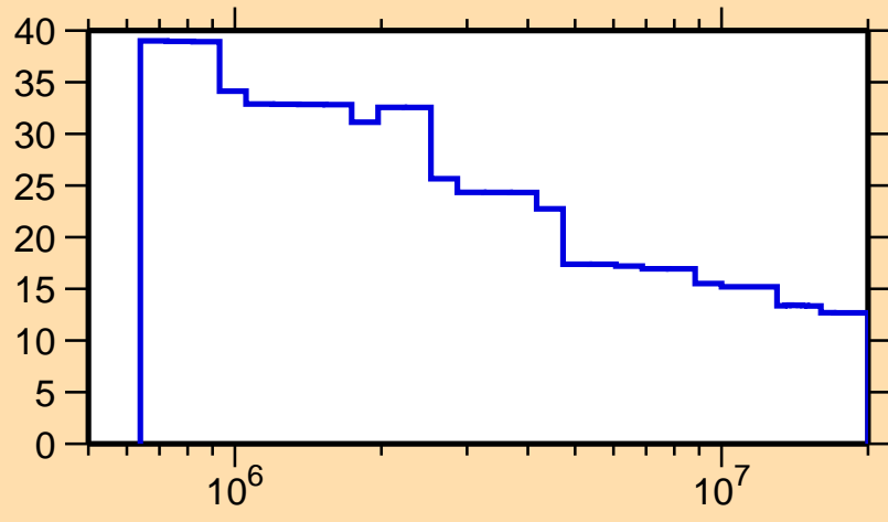
\Delta\sigma/\sigma vs. E for ^{202}\text{Bi}(n,n\text{nonel.})
