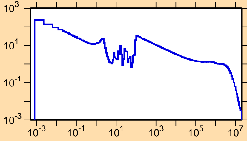
\sigma vs. E for ^{202}\text{Bi}(n,\gamma)
