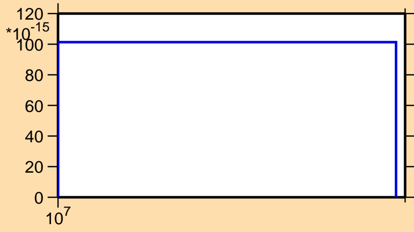
\sigma vs. E for ^{202}\text{Bi}(n,\text{pd})
