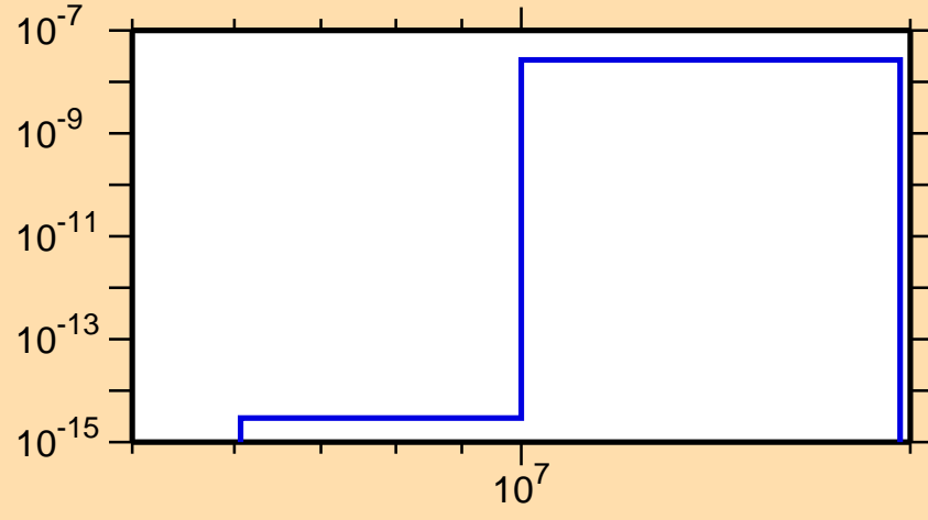
\sigma vs. E for ^{202}\text{Bi}(n,\text{He}3)
