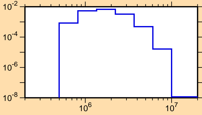
\sigma vs. E for ^{202}\text{Bi}(n,n_4)
