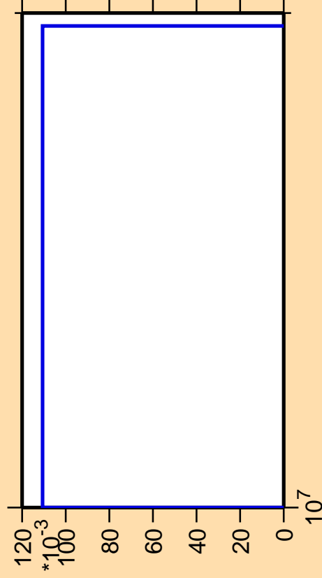
\Delta\sigma/\sigma vs. E for ^{202}\text{Bi}(\text{mt117})
