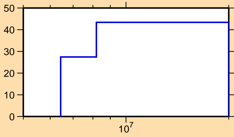
\Delta\sigma/\sigma vs. E for ^{202}\text{Bi}(n,\text{inel.})
