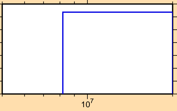
\sigma vs. E for ^{202}\text{Bi}(n,2n\alpha)
