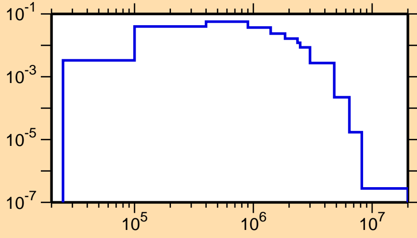
\sigma vs. E for ^{202}\text{Bi}(n,n_3)
