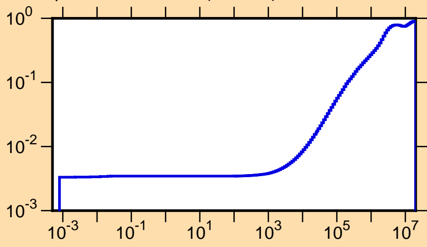
\mu vs. E for ^{203}\text{Bi}(\text{mt251})
