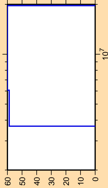
\Delta\sigma/\sigma vs. E for ^{203}\text{Bi}(n,n\alpha)
