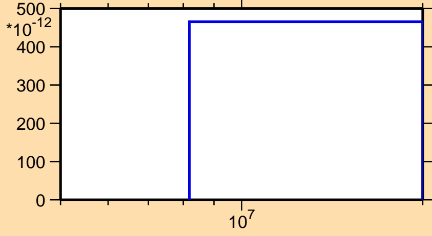
\sigma vs. E for ^{203}\text{Bi}(n,nt)
