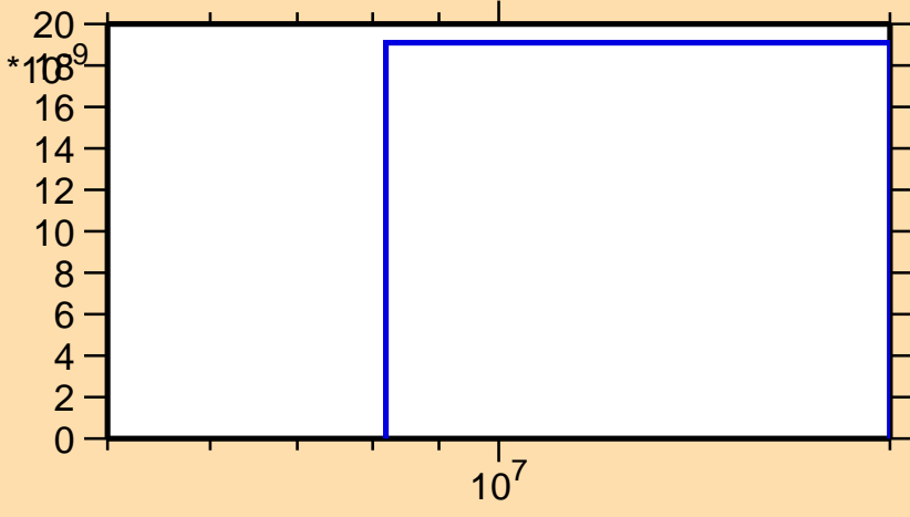
\sigma vs. E for ^{203}\text{Bi}(n,\text{nd})
