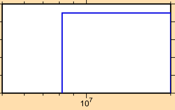
\sigma vs. E for ^{203}\text{Bi} (mt 45)
