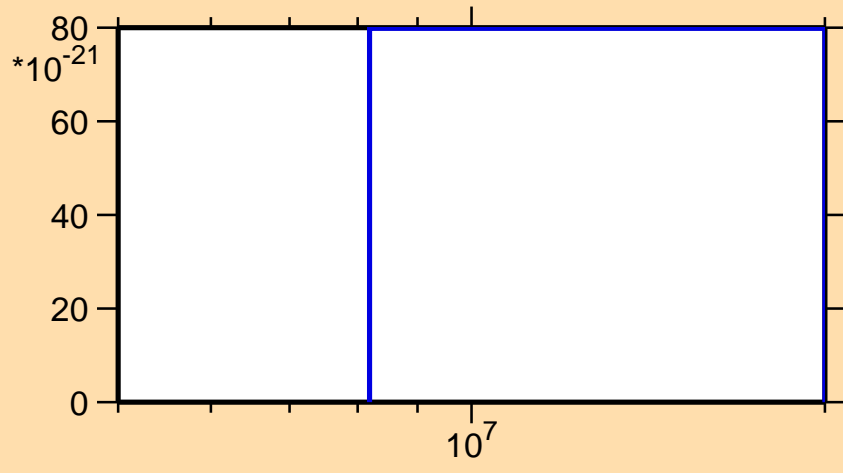
\sigma vs. E for ^{203}\text{Bi} (mt 42)
