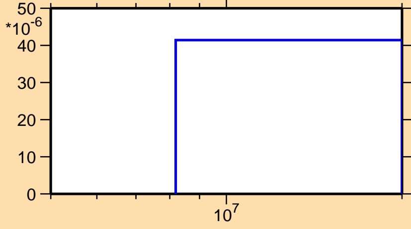
\sigma vs. E for ^{203}\text{Bi}(n,3n)
