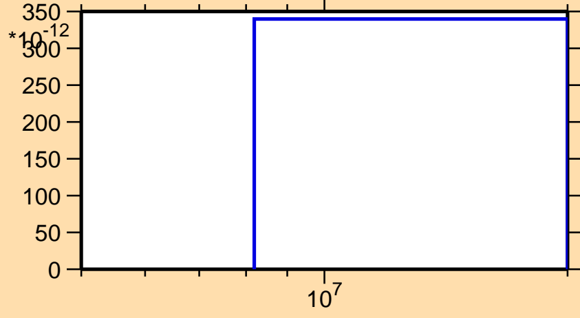
\sigma vs. E for ^{203}\text{Bi}(n,2n\alpha)
