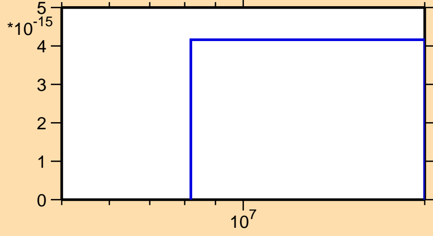
\sigma vs. E for ^{203}\text{Bi}(n,\text{pd})
