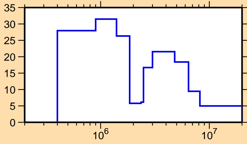
\Delta\sigma/\sigma vs. E for ^{203}\text{Bi}(n,\text{tot.})
