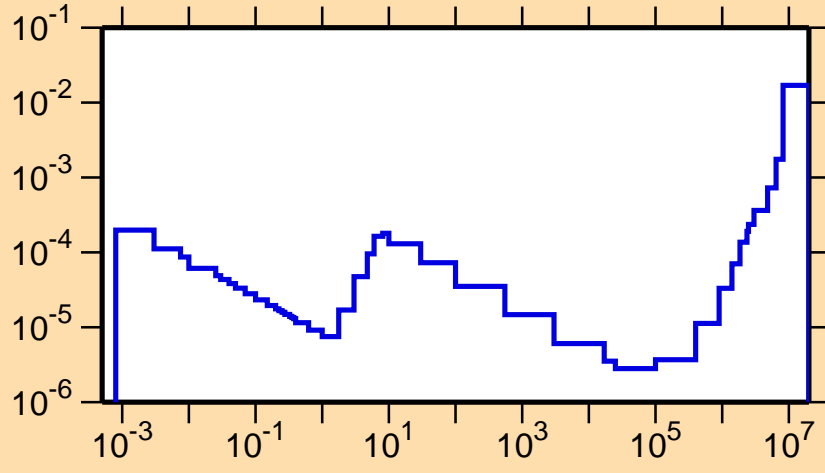
\sigma vs. E for ^{203}\text{Bi}(n,p)
