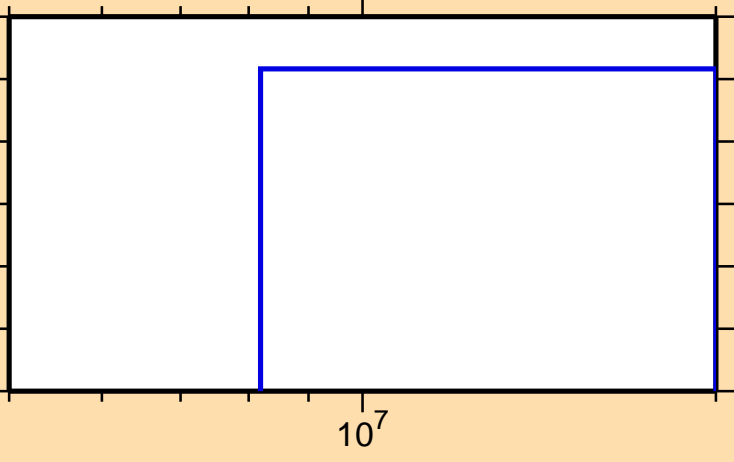
\sigma vs. E for ^{203}\text{Bi}(n,p\alpha)
