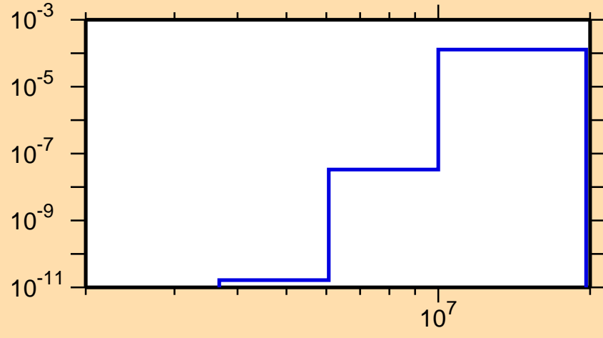
\sigma vs. E for ^{204}\text{Bi}(n,n\alpha)
