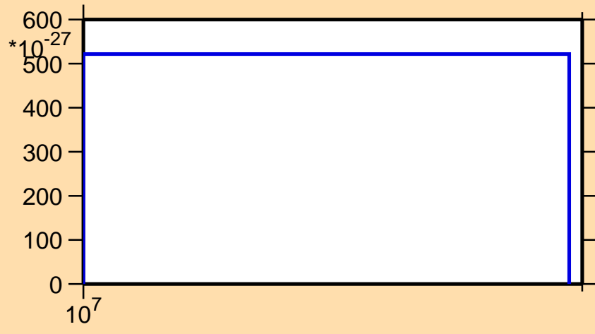
\sigma vs. E for ^{204}\text{Bi} (mt 42)
