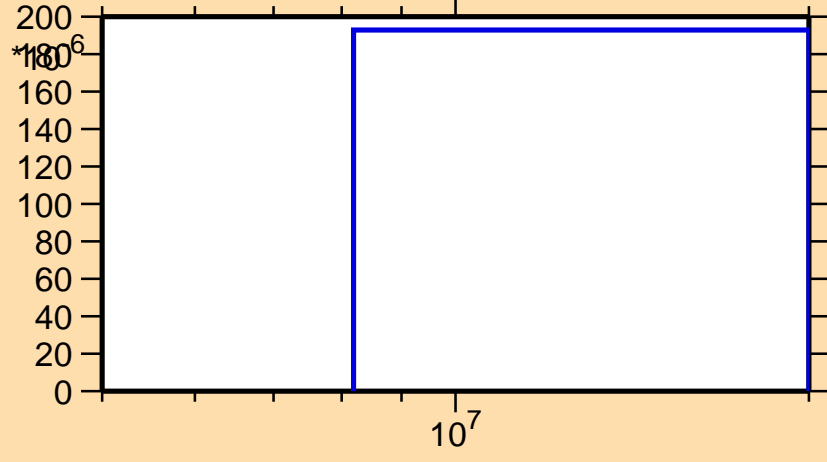
\sigma vs. E for ^{204}\text{Bi}(n,3n)
