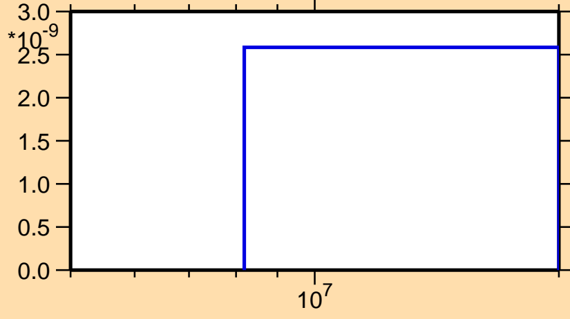
\sigma vs. E for ^{204}\text{Bi}(n,2n\alpha)
