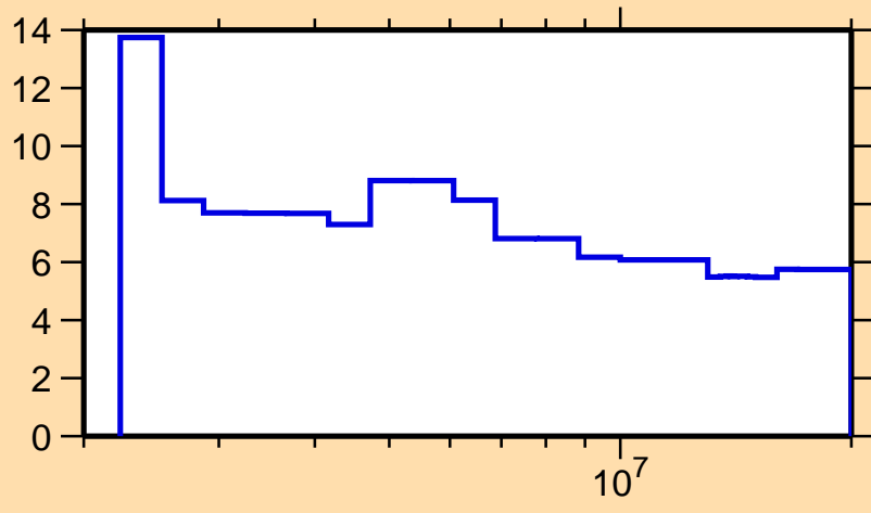
\Delta\sigma/\sigma vs. E for ^{205}\text{Bi}(n,n\text{onel.})
