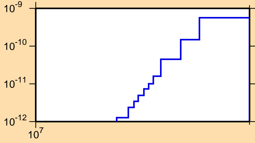
\sigma vs. E for ^{205}\text{Bi}(n,p\alpha)
