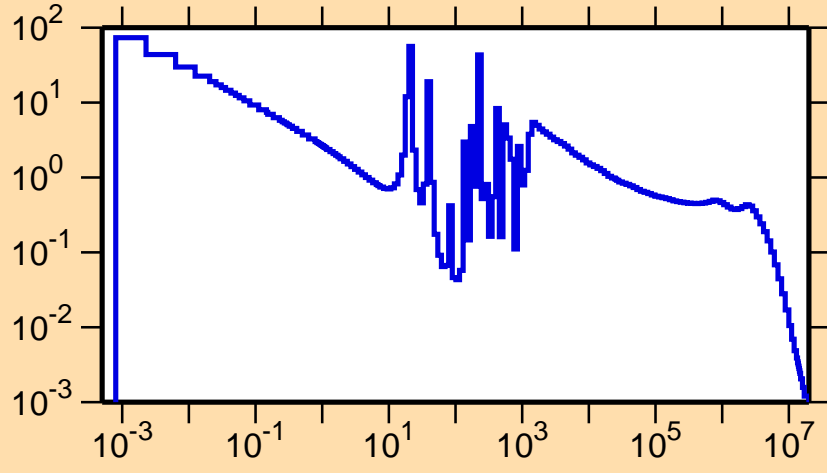
\sigma vs. E for ^{205}\text{Bi}(n,\gamma)
