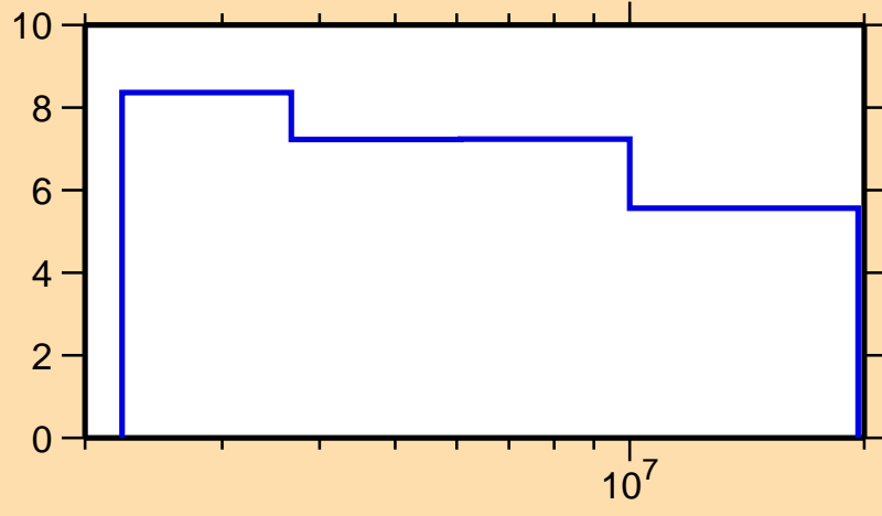
\Delta\sigma/\sigma vs. E for ^{205}\text{Bi}(n,n\text{nonel.})
