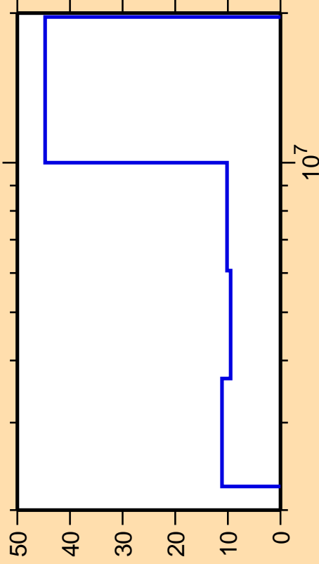
\Delta\sigma/\sigma vs. E for ^{205}\text{Bi}(n,n\text{cont.})
