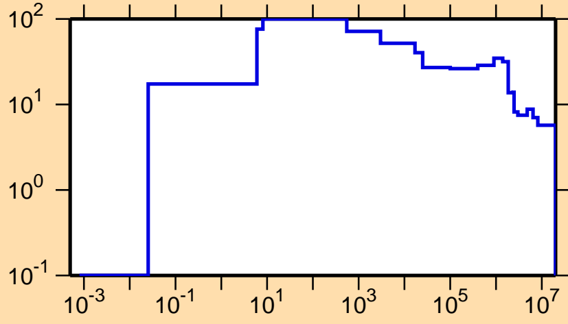
\Delta\sigma/\sigma vs. E for ^{205}\text{Bi}(n,\text{nonel.})
