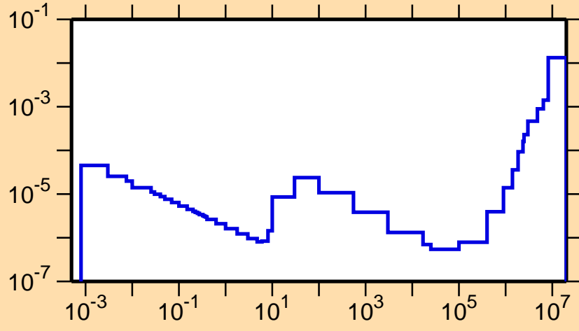
\sigma vs. E for ^{205}\text{Bi}(n,p)
