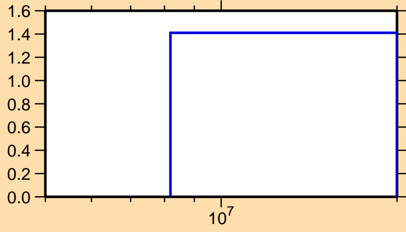
\sigma vs. E for ^{205}\text{Bi}(n,2n)
