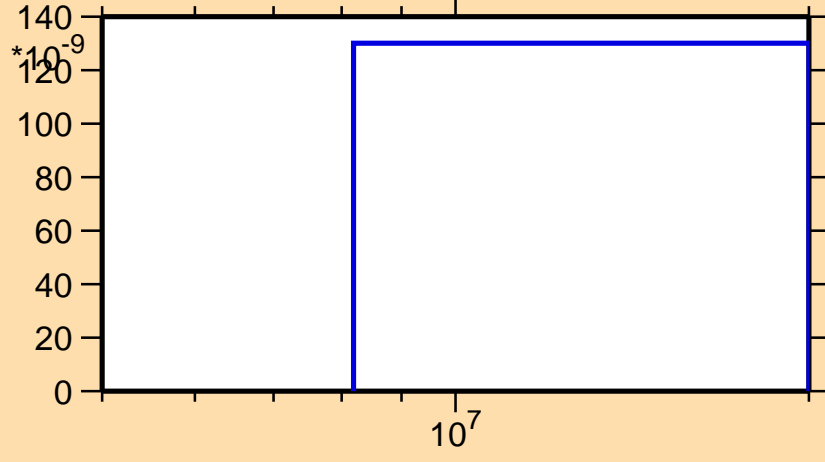
\sigma vs. E for ^{205}\text{Bi}(n,2np)
