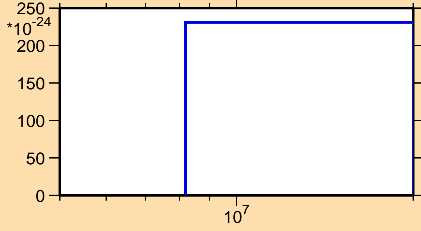
\sigma vs. E for ^{205}\text{Bi} (mt 42)
