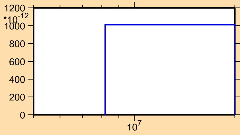
\sigma vs. E for ^{205}\text{Bi}(n,2n\alpha)
