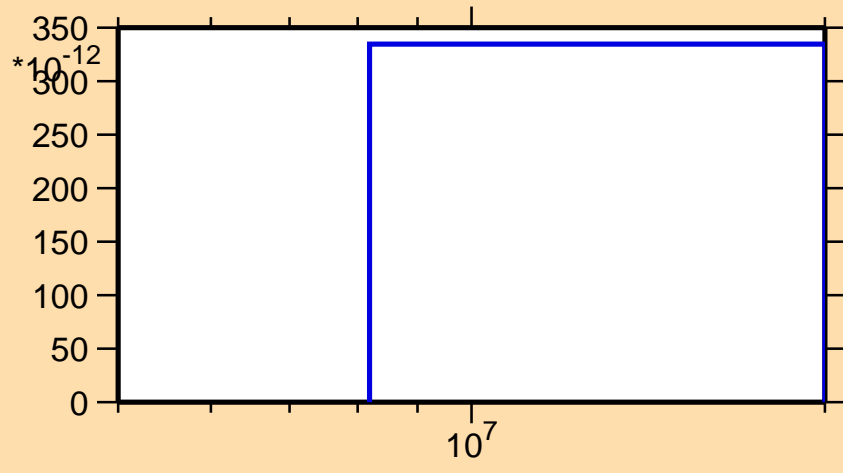
\sigma vs. E for ^{205}\text{Bi}(n,\text{He3})
