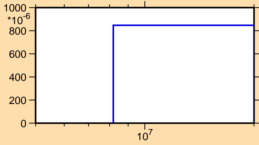
\sigma vs. E for ^{205}\text{Bi}(n,3n)
