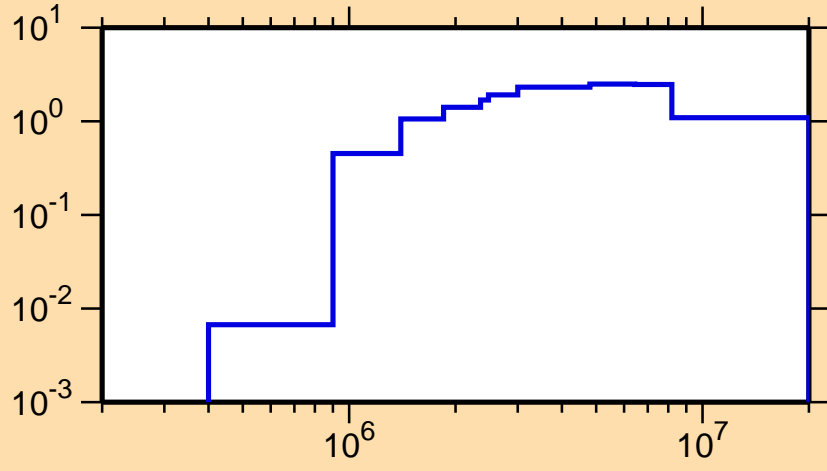
\sigma vs. E for ^{205}\text{Bi}(n,\text{inel.})
