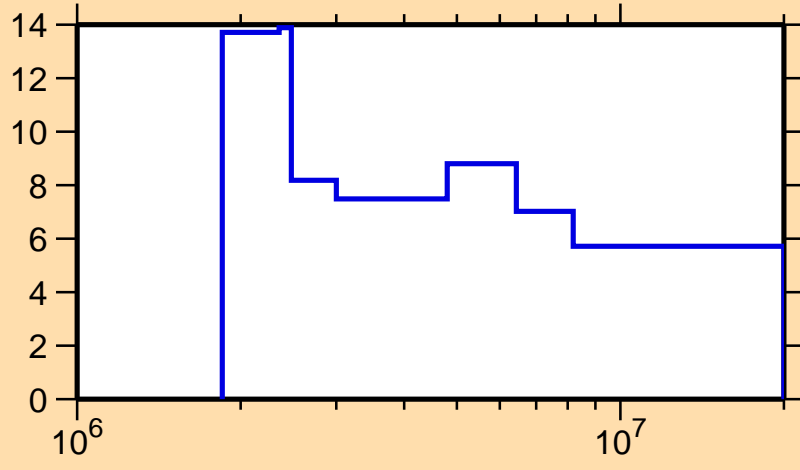
\Delta\sigma/\sigma vs. E for ^{205}\text{Bi}(n,\text{nonel.})
