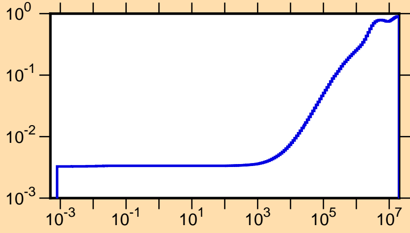
\mu vs. E for ^{206}\text{Bi}(\text{mt251})
