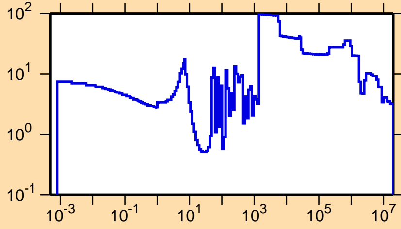
\Delta\sigma/\sigma vs. E for ^{206}\text{Bi}(n,\text{tot.})
