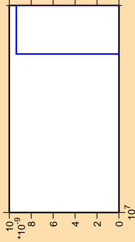
\Delta\sigma/\sigma vs. E for ^{206}\text{Bi} (mt 42)
