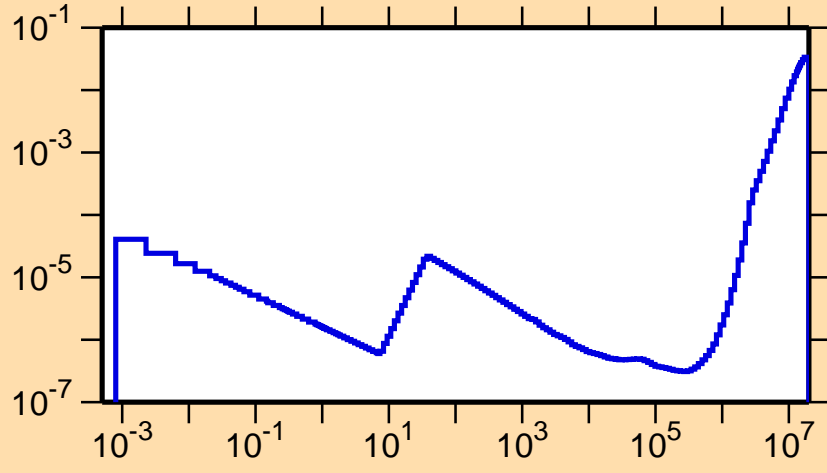
\sigma vs. E for ^{206}\text{Bi}(n,p)
