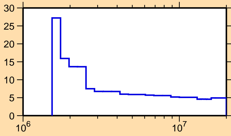
\Delta\sigma/\sigma vs. E for ^{206}\text{Bi}(n,\text{nonel.})
