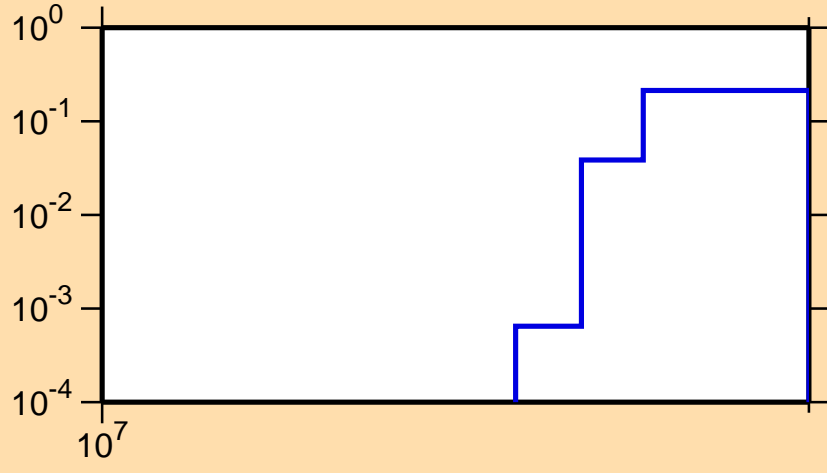
\sigma vs. E for ^{206}\text{Bi}(n,3n)
