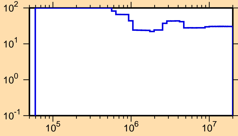
\Delta\sigma/\sigma vs. E for ^{206}\text{Bi}(n,n_1)
