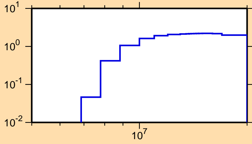
\sigma vs. E for ^{206}\text{Bi}(n,2n)
