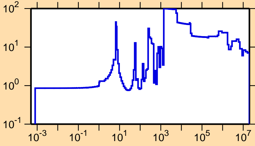
\Delta\sigma/\sigma vs. E for ^{206}\text{Bi}(n,\text{el.})
