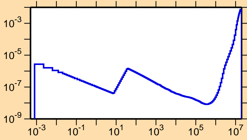
\sigma vs. E for ^{206}\text{Bi}(n,\alpha)
