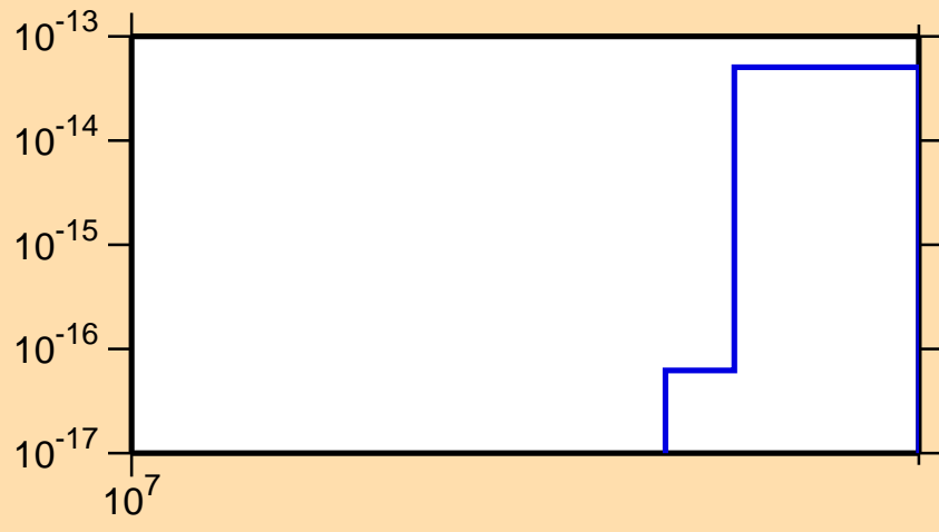
\sigma vs. E for ^{206}\text{Bi} (mt 34)
