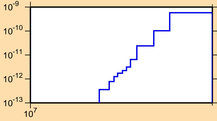
\sigma vs. E for ^{206}\text{Bi}(n,p\alpha)
