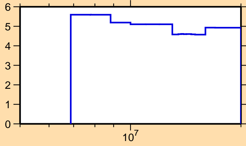
\Delta\sigma/\sigma vs. E for ^{206}\text{Bi}(n,\text{nonel.})
