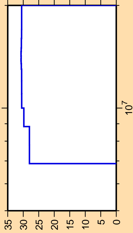
\Delta\sigma/\sigma vs. E for ^{206}\text{Bi}(n,n_1)
