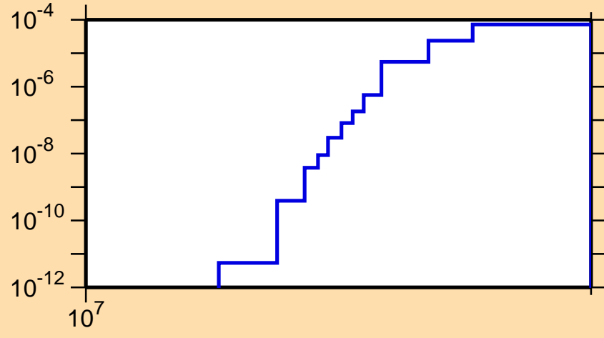
\sigma vs. E for ^{206}\text{Bi}(n,2np)
