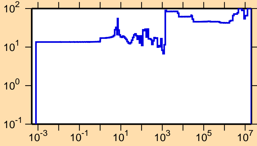
\Delta\sigma/\sigma vs. E for ^{206}\text{Bi}(n,\gamma)
