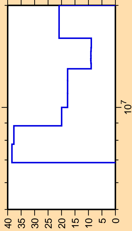
\Delta\sigma/\sigma vs. E for ^{206}\text{Bi}(n,2n)
