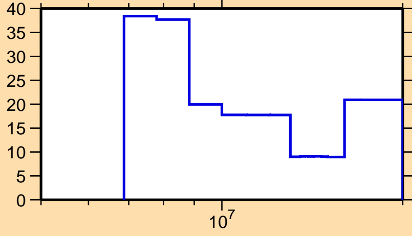
\Delta\sigma/\sigma vs. E for ^{206}\text{Bi}(n,2n)
