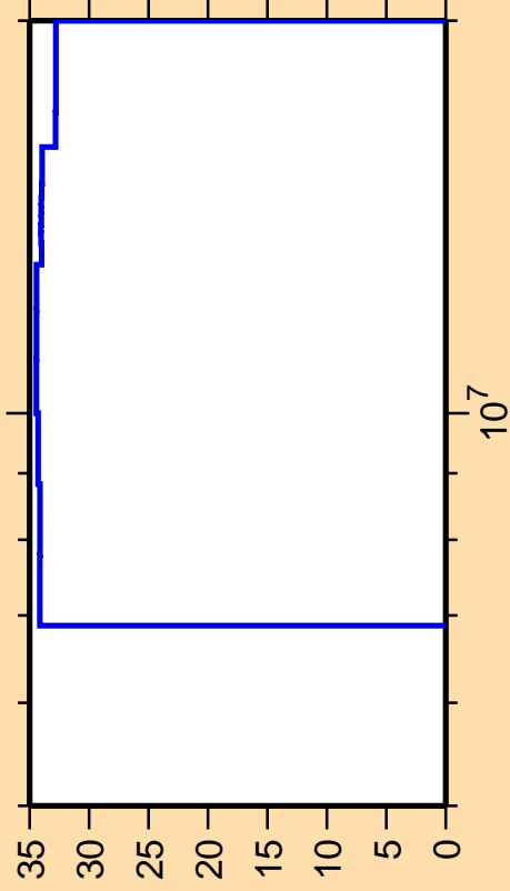
\Delta\sigma/\sigma vs. E for ^{206}\text{Bi}(n,p)
