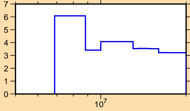
\Delta\sigma/\sigma vs. E for ^{206}\text{Bi}(n,\text{tot.})
