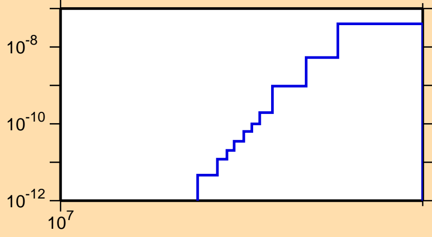
\sigma vs. E for ^{206}\text{Bi}(n,\text{He}3)
