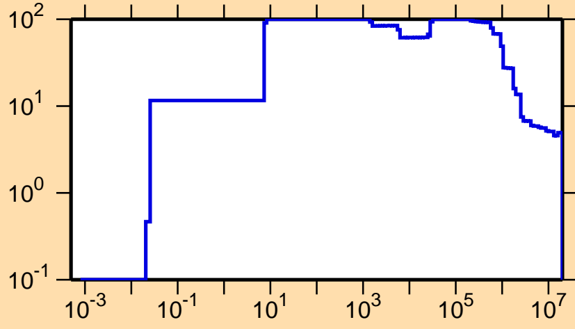
\Delta\sigma/\sigma vs. E for ^{206}\text{Bi}(n,\text{nonel.})
