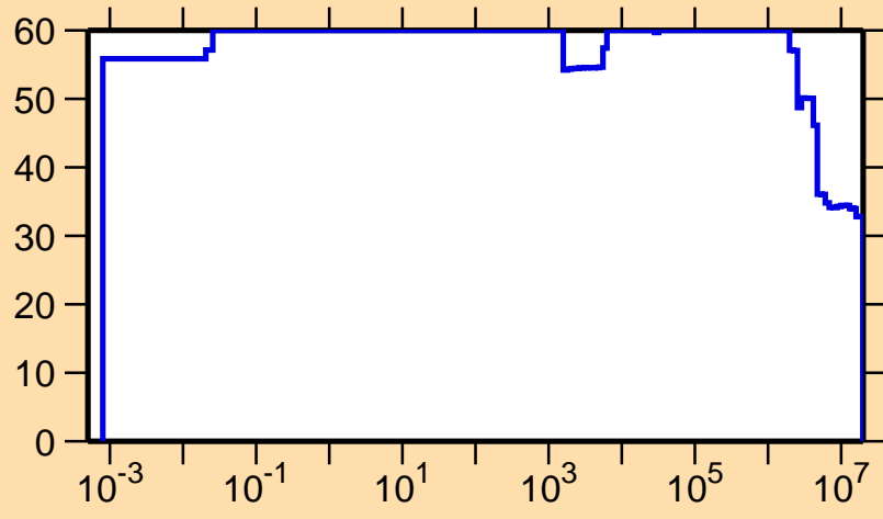
\Delta\sigma/\sigma vs. E for ^{206}\text{Bi}(n,p)
