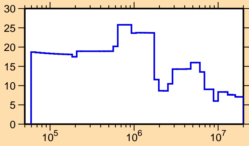
\Delta\sigma/\sigma vs. E for ^{206}\text{Bi}(n,\text{el.})
