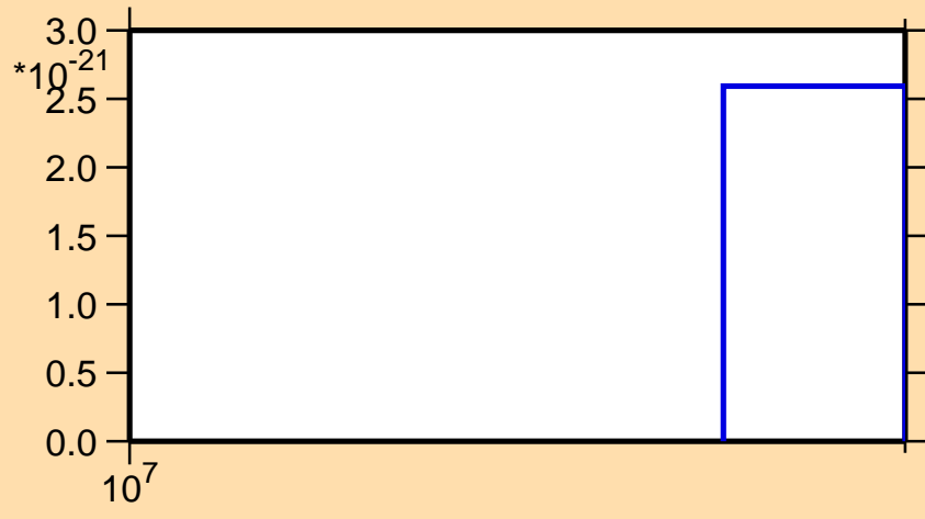
\sigma vs. E for ^{206}\text{Bi} (mt 42)
