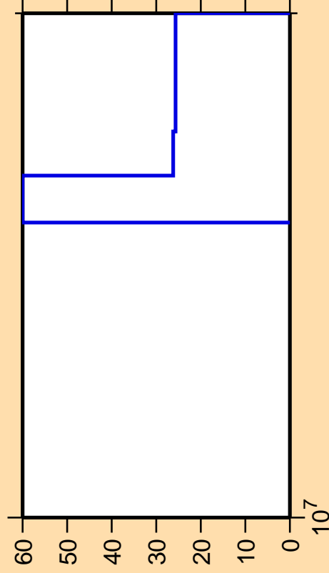
\Delta\sigma/\sigma vs. E for ^{206}\text{Bi}(n,3n)
