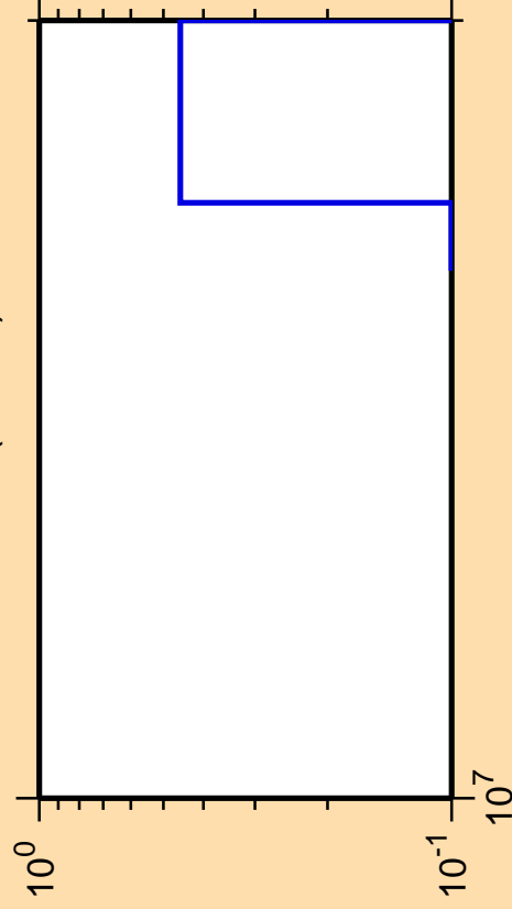
\Delta\sigma/\sigma vs. E for ^{206}\text{Bi} (mt 34)
