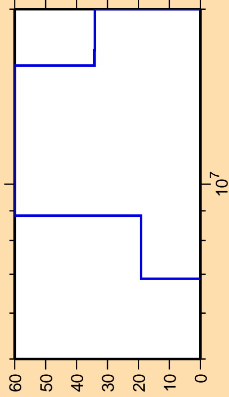
\Delta\sigma/\sigma vs. E for ^{206}\text{Bi}(n,n\text{cont.})
