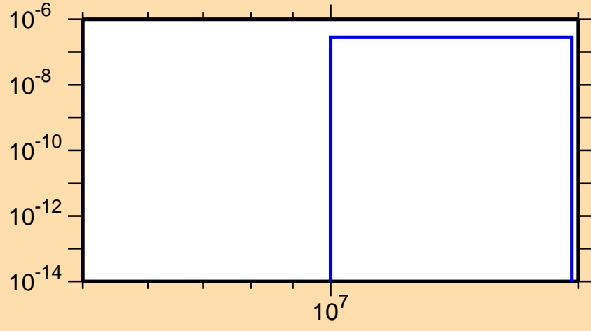
\sigma vs. E for ^{206}\text{Bi}(n,nd)
