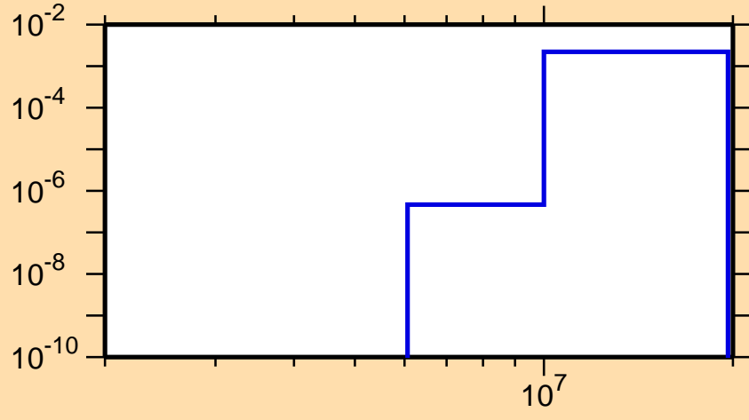
\sigma vs. E for ^{206}\text{Bi}(n,d)
