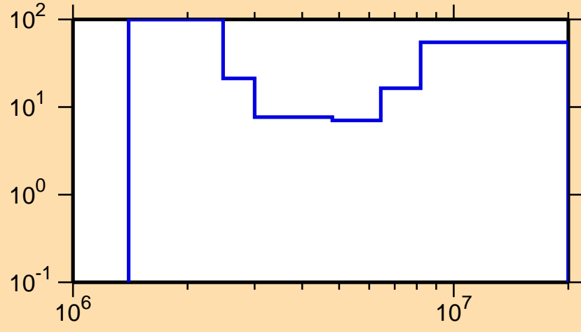
\Delta\sigma/\sigma vs. E for ^{206}\text{Bi}(n,n\text{cont.})
