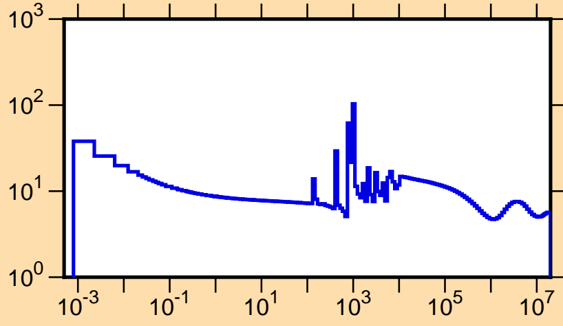
\sigma vs. E for ^{208}\text{Bi}(n,\text{tot.})
