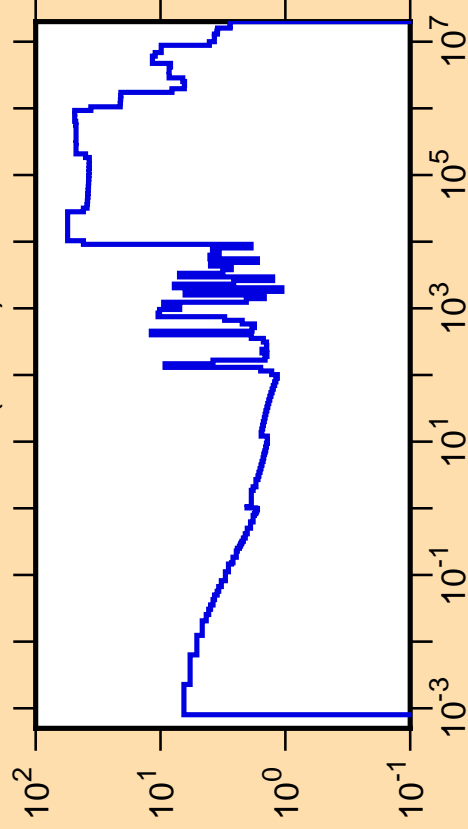
\Delta\sigma/\sigma vs. E for ^{208}\text{Bi}(n,\text{tot.})
