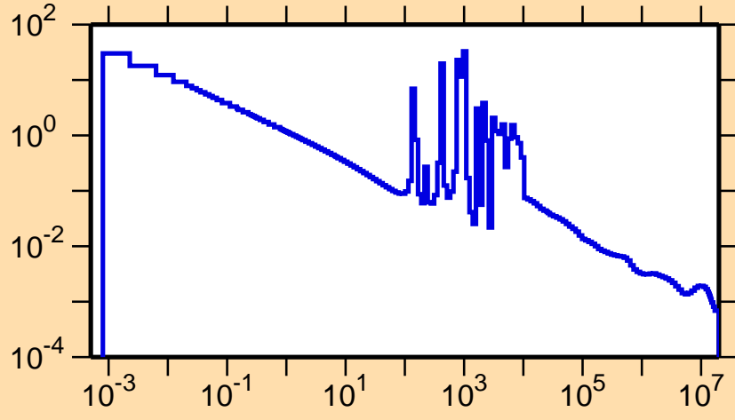
\sigma vs. E for ^{208}\text{Bi}(n,\gamma)
