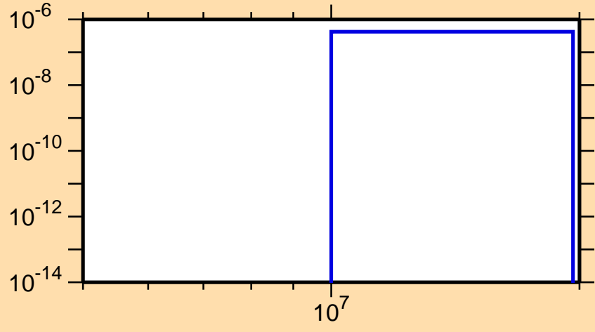
\sigma vs. E for ^{208}\text{Bi}(n,nd)
