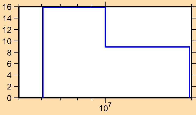
\Delta\sigma/\sigma vs. E for ^{208}\text{Bi}(n,2n)
