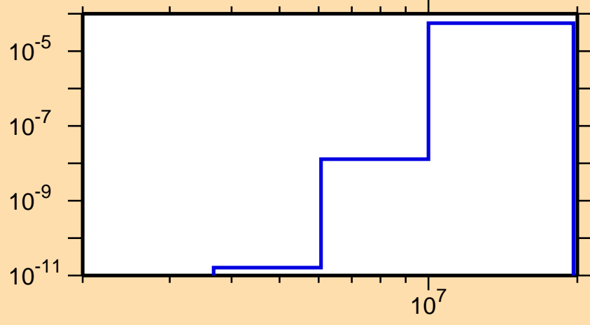
\sigma vs. E for ^{208}\text{Bi}(n,n\alpha)
