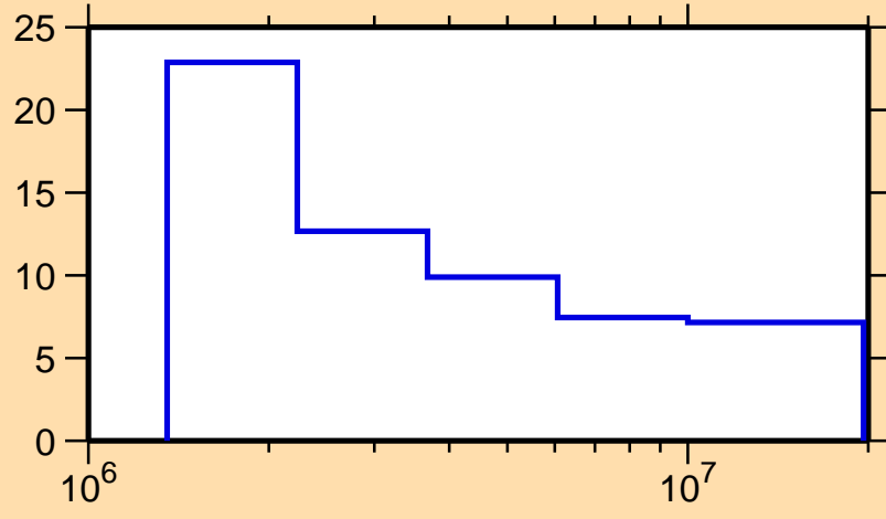
\Delta\sigma/\sigma vs. E for ^{208}\text{Bi}(n,n\text{onel.})
