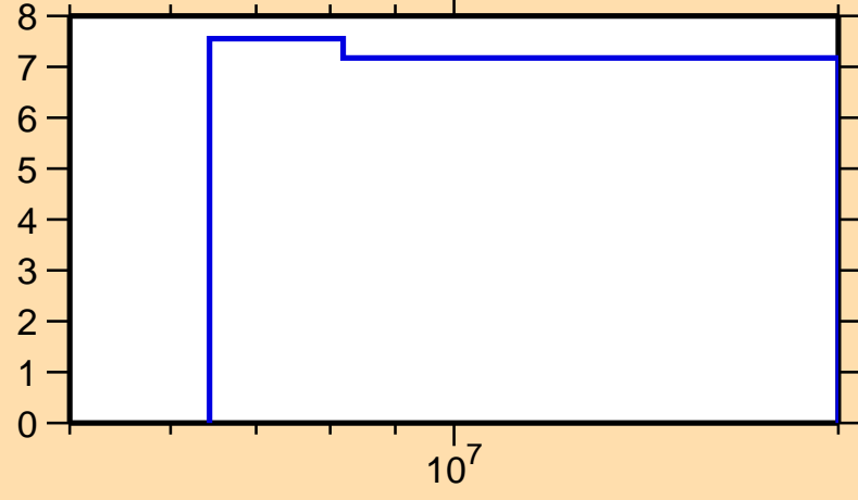
\Delta\sigma/\sigma vs. E for ^{208}\text{Bi}(n,\text{nonel.})
