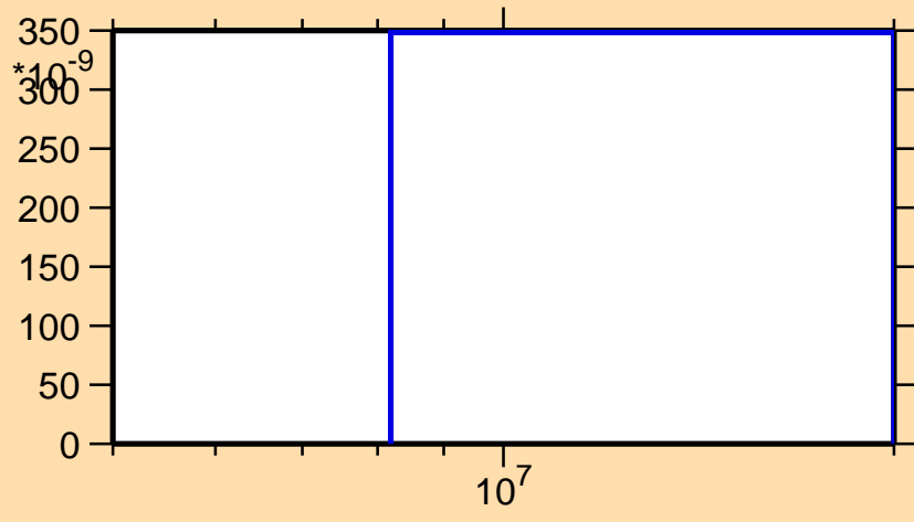
\sigma vs. E for ^{208}\text{Bi}(n,\text{nd})
