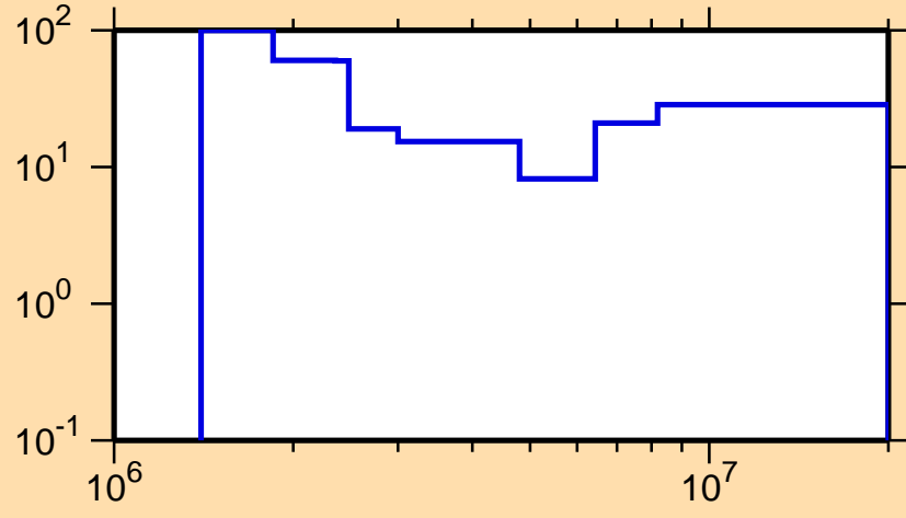
\Delta\sigma/\sigma vs. E for ^{208}\text{Bi}(n,n\text{cont.})
