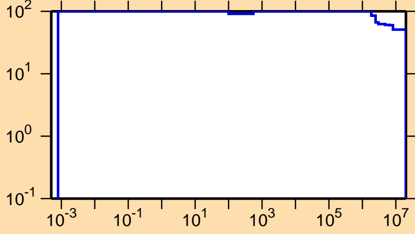
\Delta\sigma/\sigma vs. E for ^{208}\text{Bi}(n,p)
