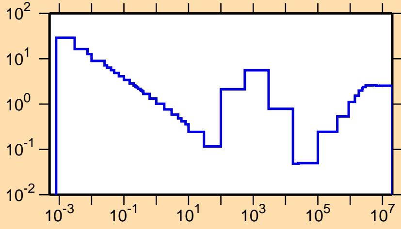
\sigma vs. E for ^{208}\text{Bi}(n,\text{nonel.})
