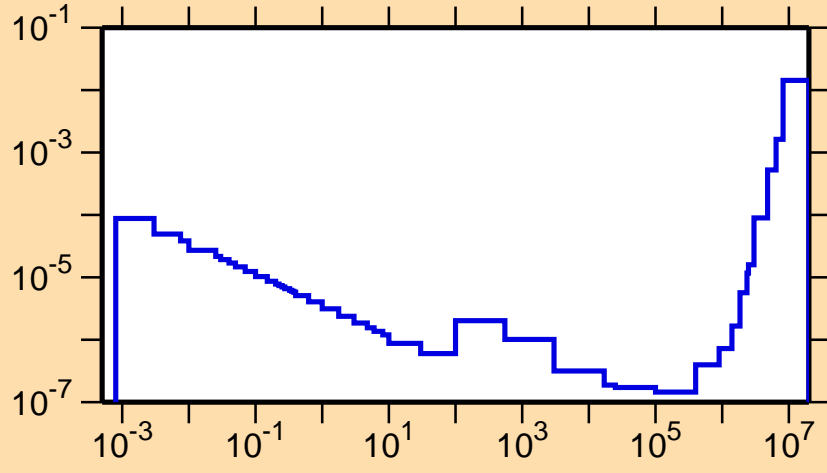
\sigma vs. E for ^{208}\text{Bi}(n,p)
