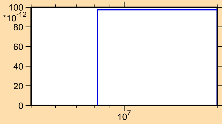
\sigma vs. E for ^{208}\text{Bi}(n,\text{He}3)
