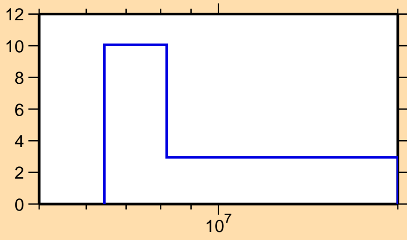
\Delta\sigma/\sigma vs. E for ^{208}\text{Bi}(n,\text{tot.})
