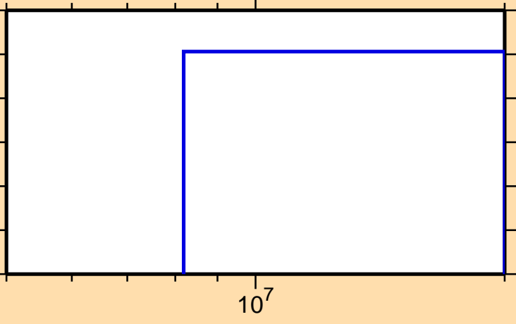
\sigma vs. E for ^{208}\text{Bi}(n,2np)
