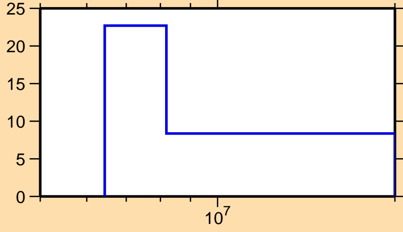
\Delta\sigma/\sigma vs. E for ^{208}\text{Bi}(n,2n)
