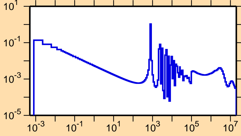
\sigma vs. E for ^{209}\text{Bi}(n,\gamma)
