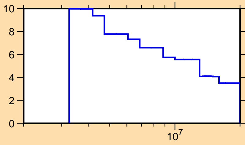
\Delta\sigma/\sigma vs. E for ^{209}\text{Bi}(n,n\text{onel.})
